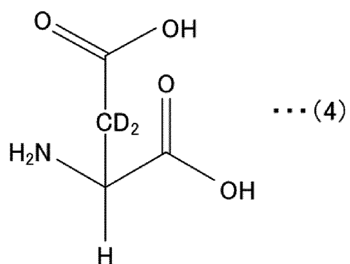
[Chem. 4]
