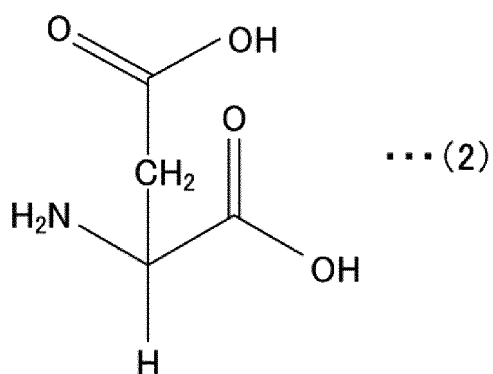
[Chem. 2]
