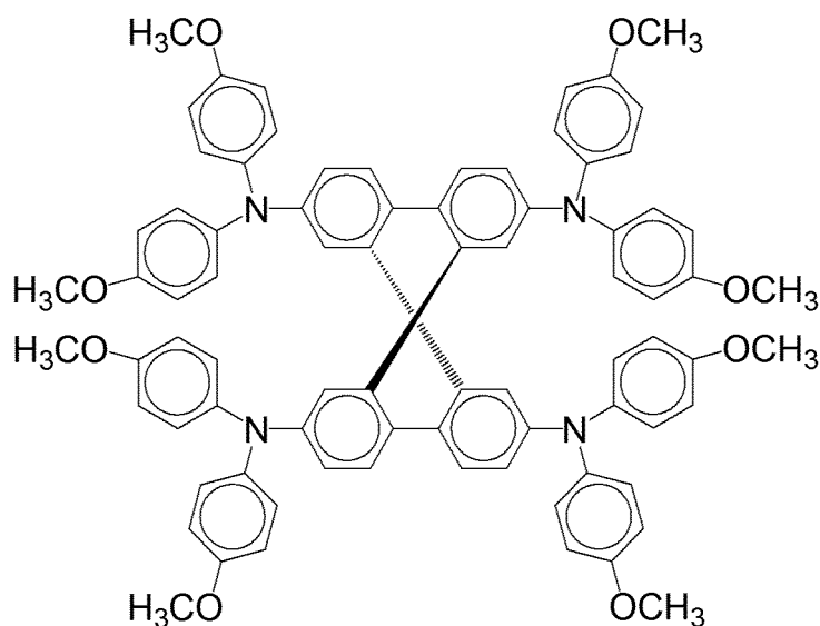
<Structural formula (1)>
