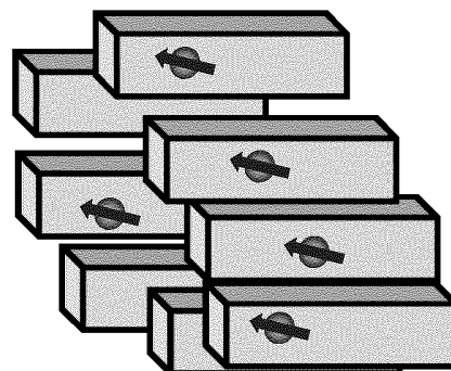
c, grating or pillars with color centers
