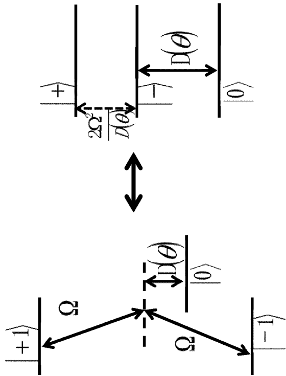
c, double quantum transition
