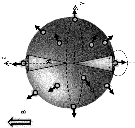
a, nanodiamond distribution in solution
