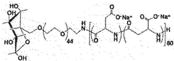
Glc(6)-PEG-P(Asp)
