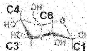
Glucose
