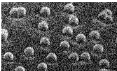
Figure 24. Nanocaps (half-nanoshells) comprising polystyrene nanospheres coated with silver
