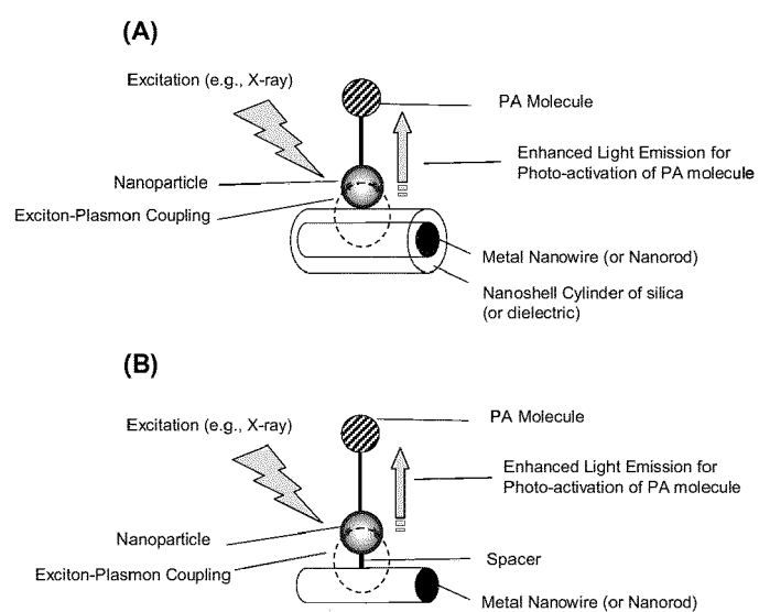
Exciton-Plasmon coupling Between Metal Nanorod and Nanoparticle
