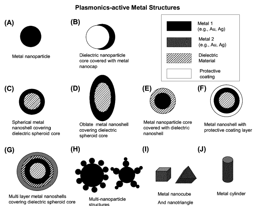
Figure 9. Plasmonics-active Nanostructures
