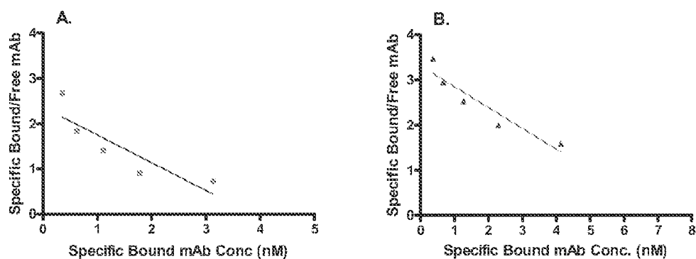
Figure 13. Scatchard Analyses: ^{125}\text{I} -radiolabelled A) ch806 and B) hu806 antibody constructs binding to A431 cells.
