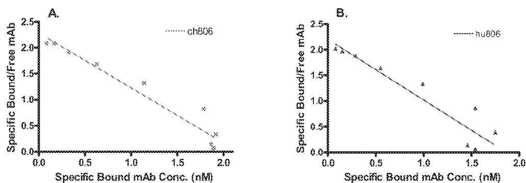
Figure 13. Scatchard Analyses: ^{125}\text{I} -radiolabelled A) ch806 and B) hu806 antibody constructs binding to A431 cells.
