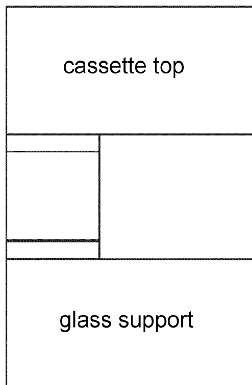
Cassette Channel (partial section view)
