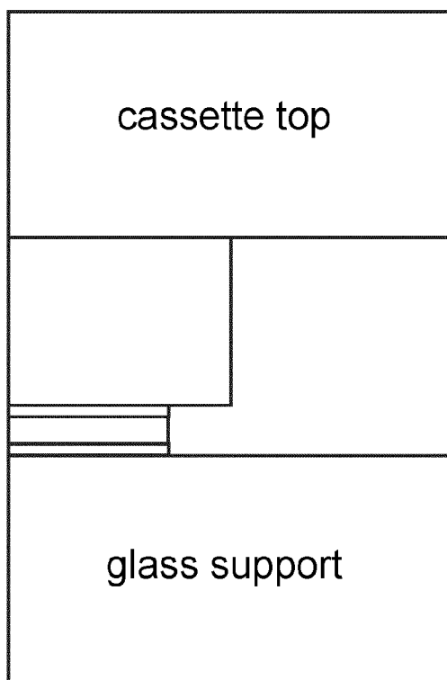
Cassette Channel (partial section view)
