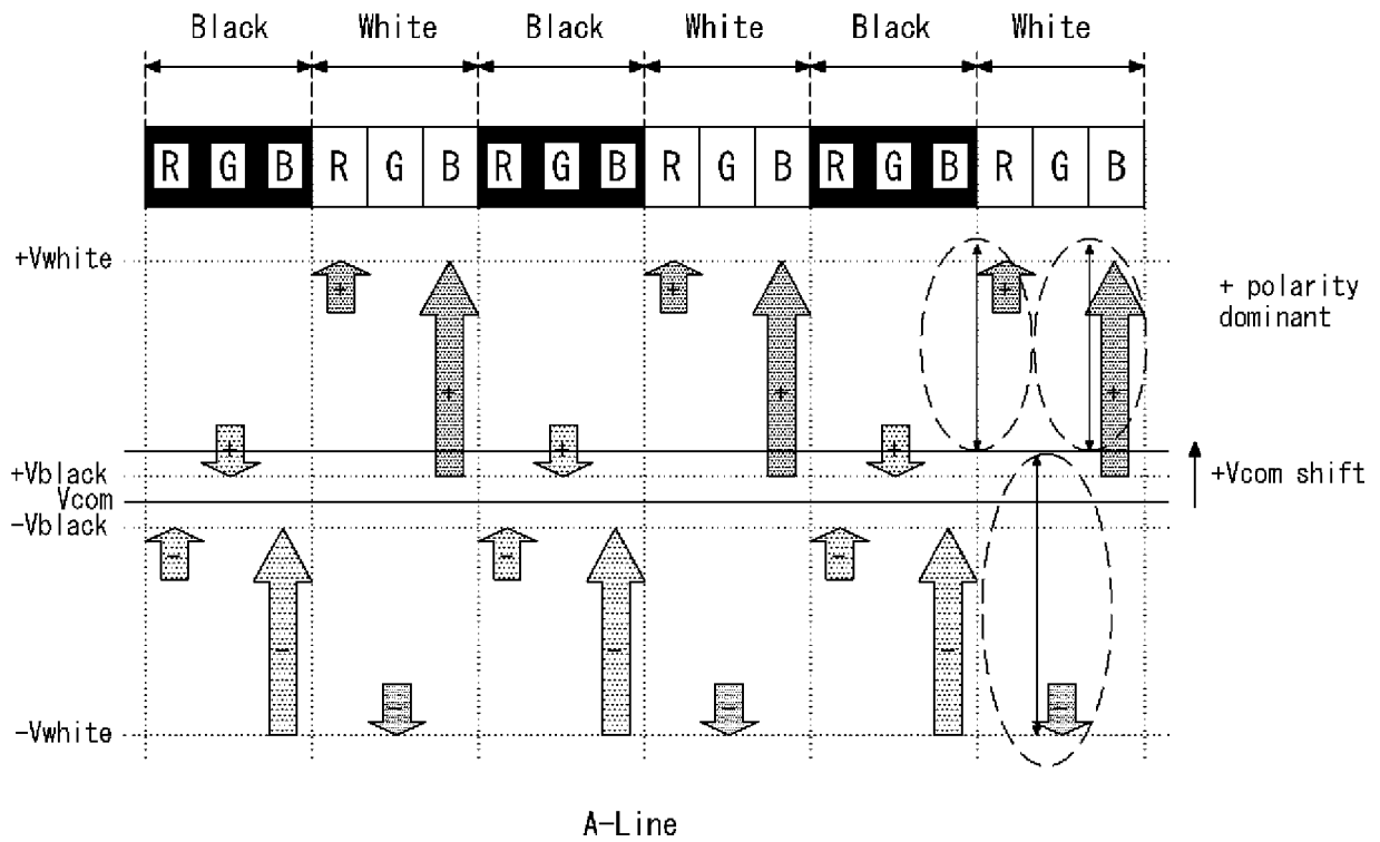
FIG. 3 (RELATED ART)
