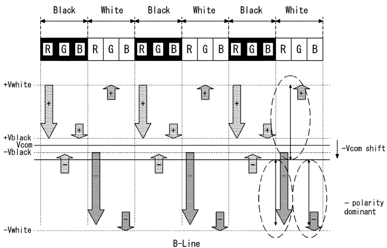
FIG. 4 (RELATED ART)
