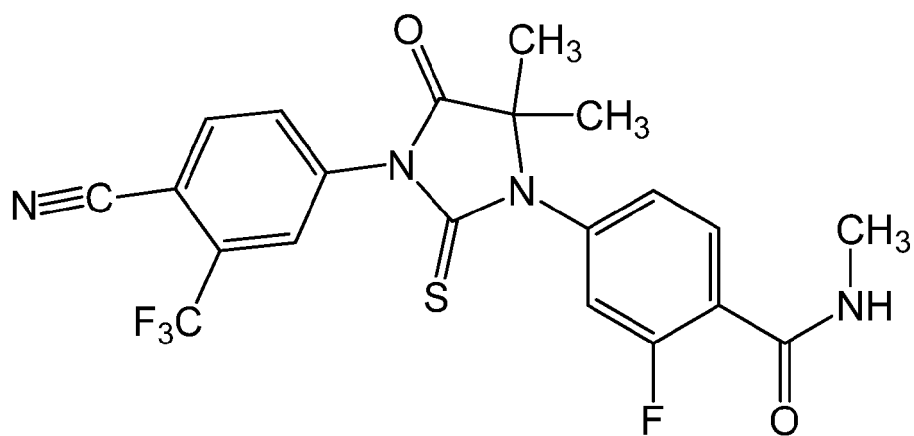
4-(3-(4-cyano-3-(trifluoromethyl)phenyl)-5,5-dimethyl-4-oxo-2-thioxoimidazolidin-1-yl)-2-fluoro-N-methylbenzamide (enzalutamide)
