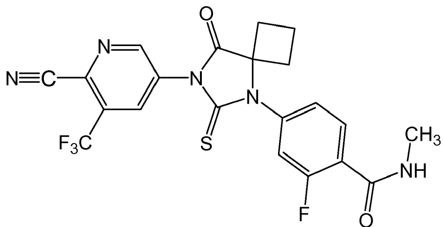
4-[7-(6-cyano-5-trifluoromethylpyridin-3-yl)-8-oxo-6-thioxo-5,7-diazaspiro[3.4]oct-5-yl]-2-fluoro-N-methylbenzamide (ARN-509)
