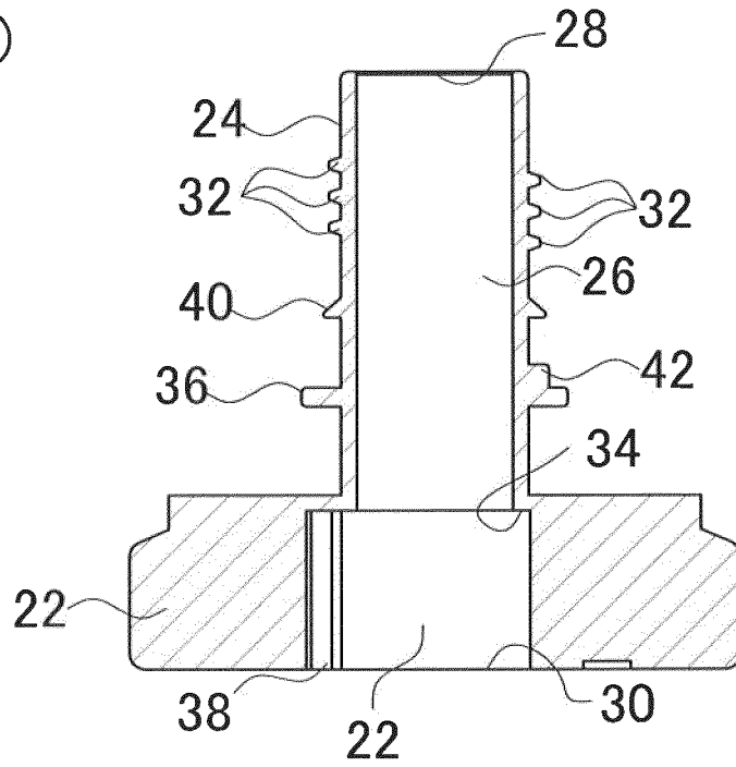
Sectional View III-III
