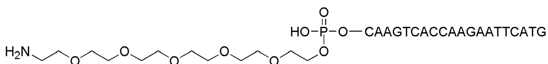
Scheme 1.2. The display oligo containing a chemical reaction site ( H_2N ), a polyethyleneglycol linker, and an oligonucleotide tag.
