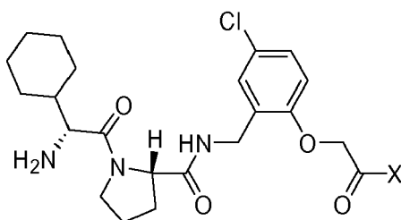
Scheme 1.5 Chemical structure corresponding to the building block combination X-REA001710-REA001712-BBA000031
