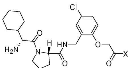
Scheme 2.4 Chemical structure corresponding to the building block combination X-REA001710-BBA001023-BBA000031
