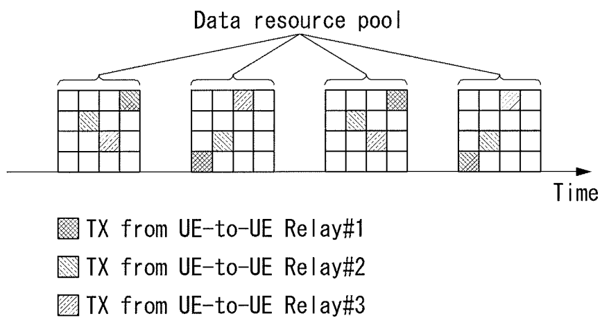
(a) Wireless resource use_type 1
