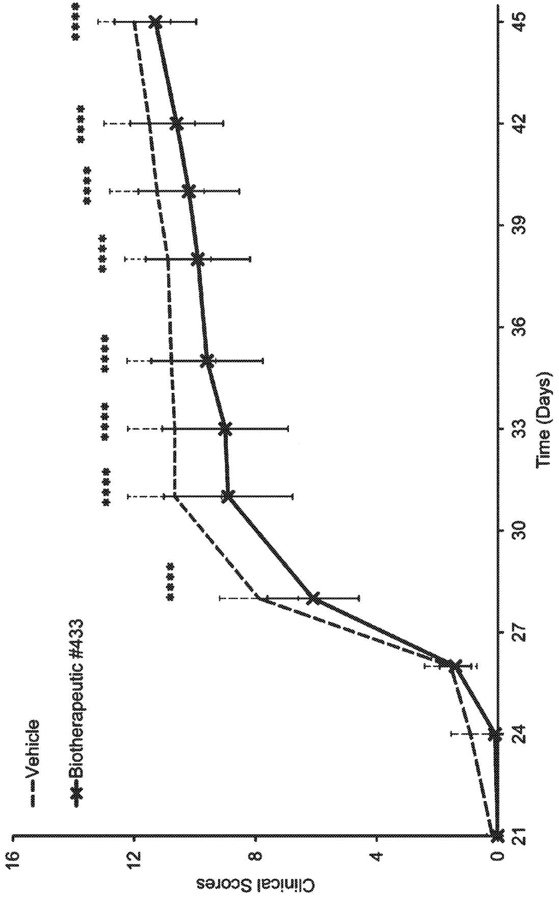
FIG. 21 Clinical Scores
