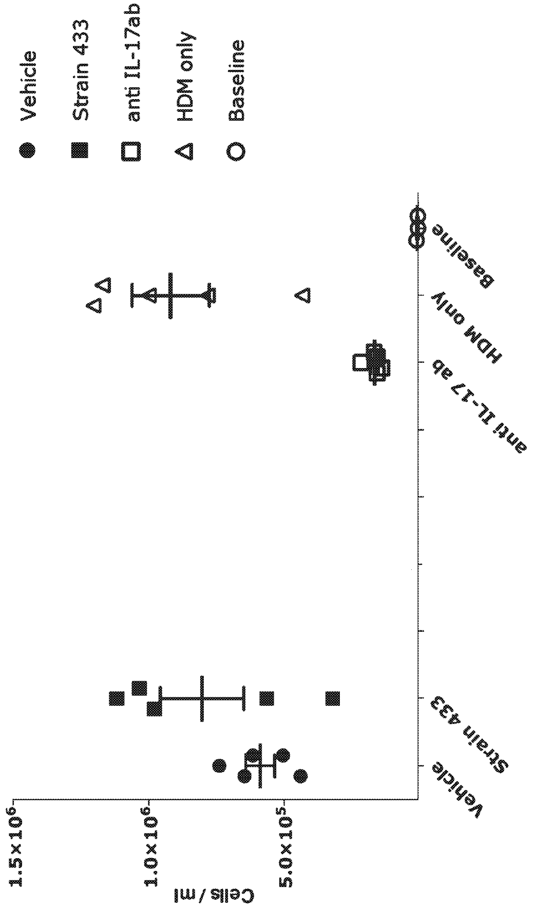
FIG. 15 Total neutrophils.
