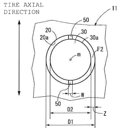
TIRE AXIAL DIRECTION TIRE RADIAL DIRECTION FIG. 3D B-B SECTION
