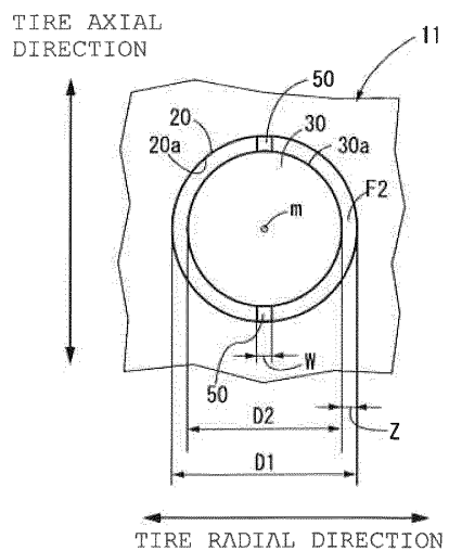
FIG. 3D B-B SECTION
