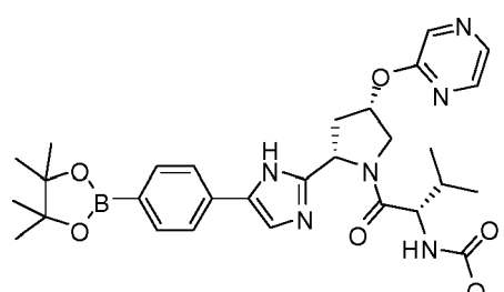
[2-Methyl-1-(4-(pyrazin-2-yloxy)-2-{5-[4-(4,4,5,5-tetramethyl-1,3,2)dioxaborolan-2-yl]-phenyl]-1 H -imidazol-2-yl]-pyrrolidine-1-carboxyl)-propyl]-carbamic acid methyl ester
