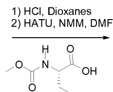
2-Methoxycarbonylamino-butyl carboxylic acid
