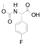
(S)-(4-Fluoro-phenyl)- methoxycarbonylamino-acetic acid
