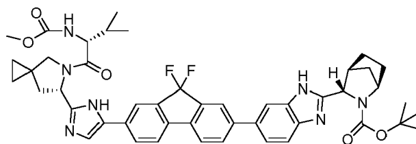
3-[6-(9,9-Difluoro-7-{2-[5-(2-methoxycarbonylamino-3-methyl-butyl)-5-aza-spiro[2.4]hept-6-yl]-3H-imidazol-4-yl]-9H-fluoren-2-yl)-1H-benzimidazol-2-yl]-2-aza-bicyclo[2.2.1]heptane-2-carboxylic acid tert -butyl ester
