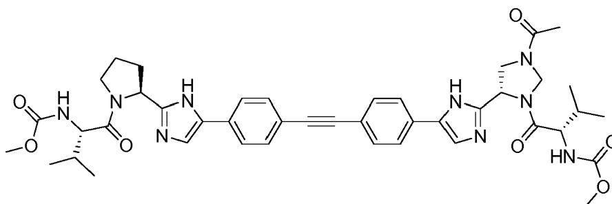
(1-{2-[5-(4-{4-[1'-Acetyl-3'-(2-methoxycarbonylamino-3-methyl-butyl)-2',3',4',5'-tetrahydro-3H,1'H-[2,4']biimidazolyl-4-yl]-phenylethynyl)-phenyl]-1H-imidazol-2-yl]-pyrrolidine-1-carbonyl}-2-methyl-propyl)-carbamic acid methyl ester
