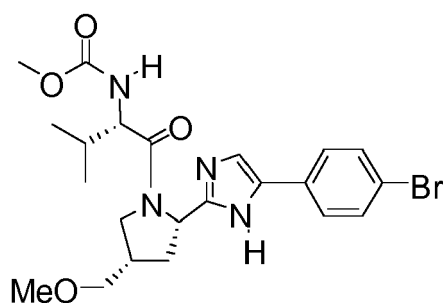
(1-{2-[5-(4-Bromo-phenyl)-1 H -imidazol-2-yl]-4-methoxymethyl-pyrrolidine-1-carbonyl}-2-methyl-propyl)-carbamic acid methyl ester
