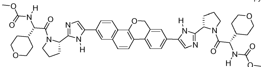
[2-(2-{5-[2-(2-{1-[2-Methoxycarbonylamino-2-(tetrahydro-pyran-4-yl)-acetyl]-pyrrolidin-2-yl]-3 H -imidazol-4-yl]-6 H -dibenzo[ c,h ]chromen-8-yl]-1 H -imidazol-2-yl]-pyrrolidin-1-yl)-2-oxo-1-(tetrahydro-pyran-4-yl)-ethyl]-carbamic acid methyl ester
