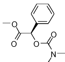
Dimethylcarbamoyloxy-phenyl-acetic acid methyl ester
