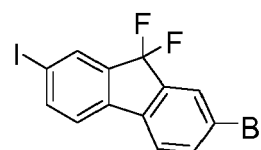
2-Bromo-9,9-difluoro-7-iodo-9 H -fluorene
