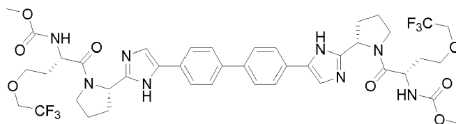
[1-(2-{5-[4'-(2-{1-[2-Methoxycarbonylamino-4-(2,2,2-trifluoro-ethoxy)-butyryl]-pyrrolidin-2-yl}-3H-imidazol-4-yl)-biphenyl-4-yl]-1H-imidazol-2-yl}-pyrrolidine-1-carbonyl)-3-(2,2,2-trifluoro-ethoxy)-propyl]-carbamic acid methyl ester
