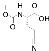
(S)-4-Cyano-2-methoxycarbonyl- aminobutyric acid
