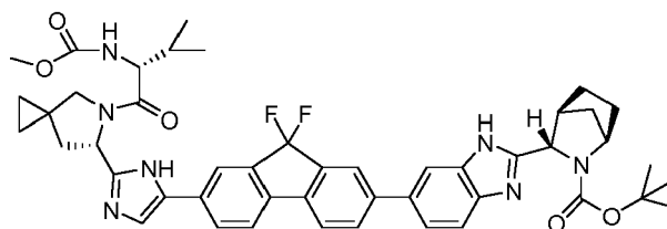
3-[6-(9,9-Difluoro-7-{2-[5-(2-methoxycarbonylamino-3-methyl-butyryl)-5-aza-spiro[2.4]hept-6-yl]-3H-imidazol-4-yl]-9H-fluoren-2-yl]-1H-benzimidazol-2-yl]-2-aza-bicyclo[2.2.1]heptane-2-carboxylic acid tert -butyl ester
