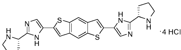
2-[5-(6-{2-[pyrrolidin-2-yl]-3 H -imidazol-4-yl})benzo[1,2- b :4,5- b' ]dithiophene-2-yl)-1 H -imidazol-2-yl]pyrrolidine tetrahydrochloride
