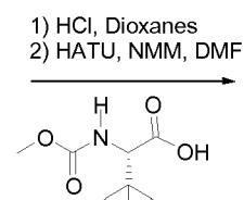
2-Methoxycarbonylamino-3,3-dimethyl-butyl carboxylic acid
