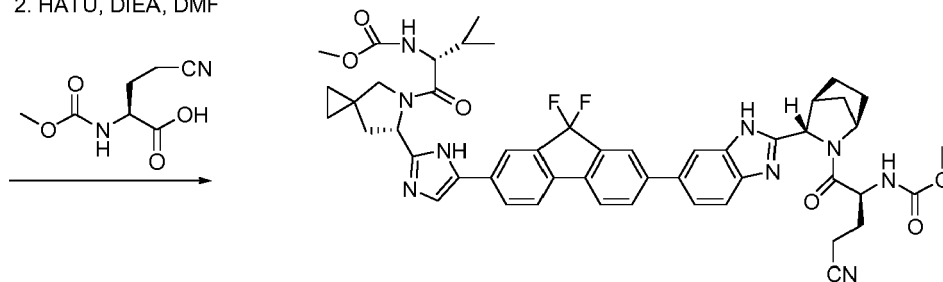
(3-Cyano-1-{3-[6-(9,9-difluoro-7-{2-[5-(2-methoxycarbonylamino-3-methyl-butyryl)-5-aza-spiro[2.4]hept-6-yl]-3H-imidazol-4-yl]-9H-fluoren-2-yl]-1H-benzimidazol-2-yl]-2-aza-bicyclo[2.2.1]heptane-2-carbonyl)-propyl)-carbamic acid methyl ester
