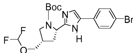
2-[5-(4-Bromo-phenyl)-1 H -imidazol-2-yl]-4-difluoromethoxymethyl-pyrrolidine-1-carboxylic acid tert -butyl ester
