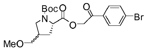
4-Methoxymethyl-pyrrolidine-1,2-dicarboxylic acid 2-[2-(4-bromo-phenyl)-2-oxo-ethyl] ester 1- tert -butyl ester
