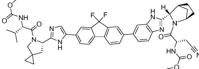
(1-{6-[5-(7-{2-[2-(3-Cyano-2-methoxycarbonylamino-propionyl)-2-aza-bicyclo[2.2.1]hept-3-yl]-3 H -benzoimidazol-5-yl]-9,9-difluoro-9 H -fluoren-2-yl}-1 H -imidazol-2-yl)-5-aza-spiro[2.4]heptane-5-carbonyl]-2-methyl-propyl)-carbamic acid methyl ester
