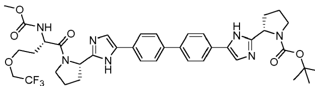
2-{5-[4'-(2-{1-[2-Methoxycarbonylamino-4-(2,2,2-trifluoroethoxy)-butyryl]-pyrrolidin-2-yl}-3H-imidazol-4-yl)-biphenyl-4-yl]-1H-imidazol-2-yl}-pyrrolidine-1-carboxylic acid tert -butyl ester
