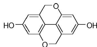
5,10-Dihydro-chromeno [5,4,3- cde ]chromene-2,7-diol
