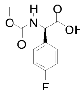
( R )-(4-Fluoro-phenyl)-methoxycarbonylamino-acetic acid
