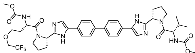
[1-(2-{5-[4'-(2-{1-[2-Methoxycarbonylamino-4-(2,2,2-trifluoro-ethoxy)-butyryl]-pyrrolidin-2-yl}-3H-imidazol-4-yl)-biphenyl-4-yl]-1H-imidazol-2-yl}-pyrrolidine-1-carbonyl)-2-methyl-propyl]-carbamic acid methyl ester
