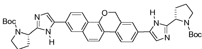
(1-{2-[5-(2-{2-[1-(carboxylic acid tert -butyl ester)-pyrrolidin-2-yl]-3 H -imidazol-4-yl]-6 H -dibenzo[ c,h ]chromen-8-yl]-1 H -imidazol-2-yl]-pyrrolidine-1-carboxylic acid tert -butyl ester
