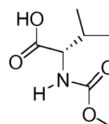
2-Methoxycarbonylamino-3-methyl-butyric acid
