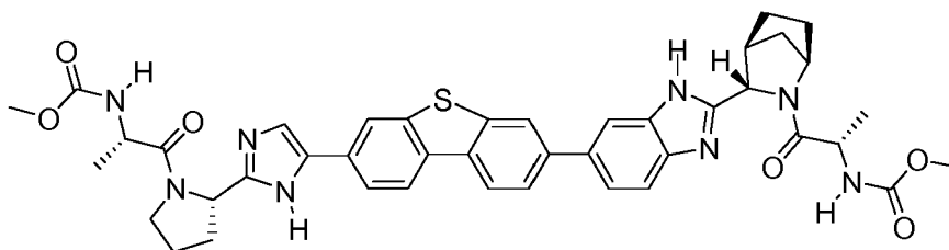
(2-{2-[5-(7-{2-[2-(2-Methoxycarbonylamino-propionyl)-2-aza-bicyclo[2.2.1]hept-3-yl]-3 H -benzoimidazol-5-yl]-dibenzothiophen-3-yl}-1 H -imidazol-2-yl]-pyrrolidin-1-yl}-1-methyl-2-oxo-ethyl)-carbamic acid methyl ester
