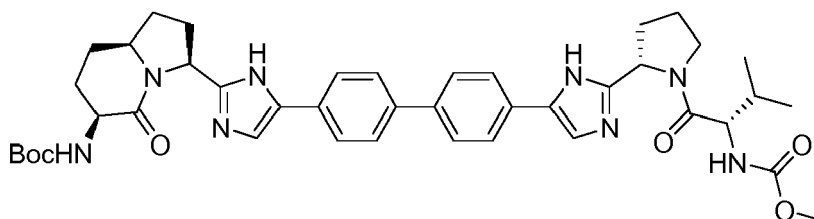
{3-[5-(4'-(2-[1-(2-Methoxycarbonylamino-3-methyl-butyl)-pyrrolidin-2-yl]-3H-imidazol-4-yl)-biphenyl-4-yl)-1H-imidazol-2-yl]-5-oxo-octahydro-indolizin-6-yl}-carbamic acid tert -butyl ester
