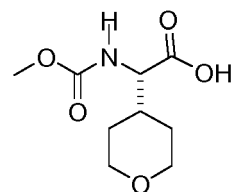
Methoxycarbonylamino-(tetrahydro-pyran-4-yl)-acetic acid
