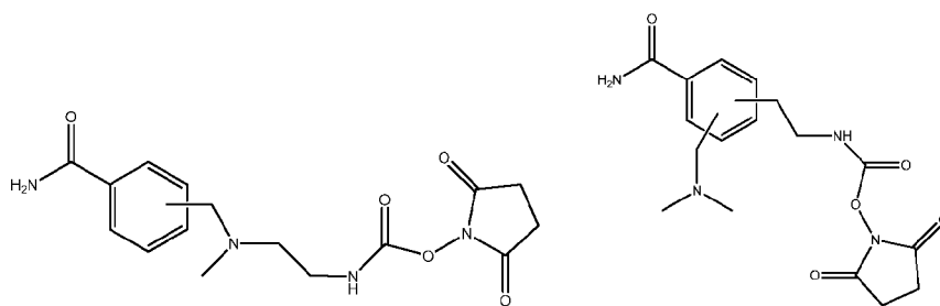
2,5-dioxopyrrolidin-1-yl 4-((2-(diethylamino)ethyl)carbamoyl)phenyl carbamate and
