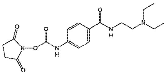
2,5-dioxopyrrolidin-1-yl 4-((2-(diethylamino)ethyl)carbamoyl)phenyl carbamate and
