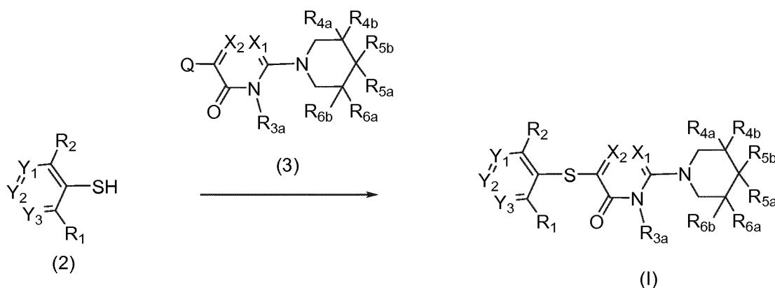
Reaction Scheme I:
