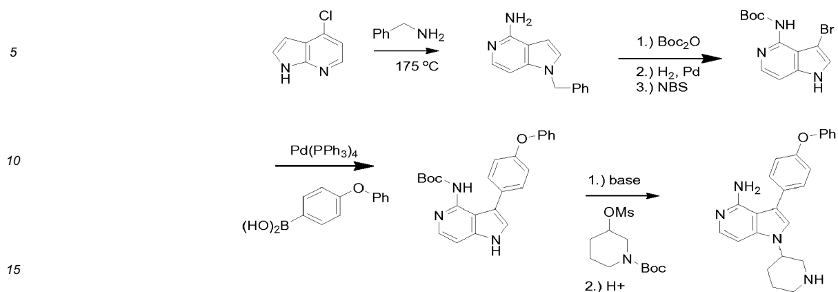
Scheme V.
