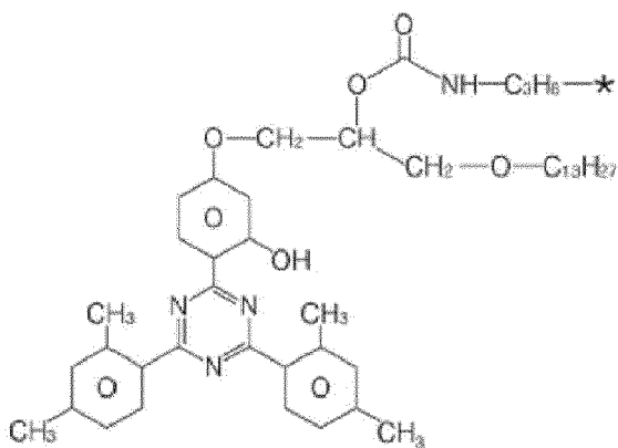
Chemical Formula iii
