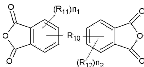
Chemical Formula 6
