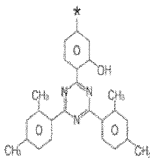
Chemical Formula 4-1
