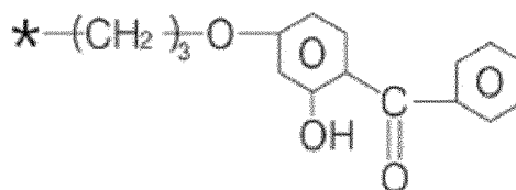
Chemical Formula ii
