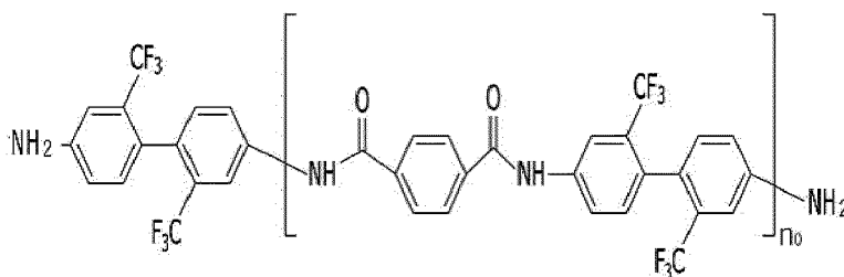
Chemical Formula 12
