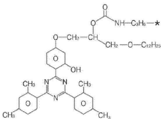
Chemical Formula iii
