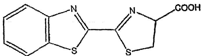
6' deoxyluciferin
