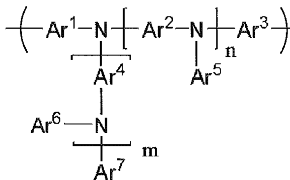
[Chemical Formula 3]
