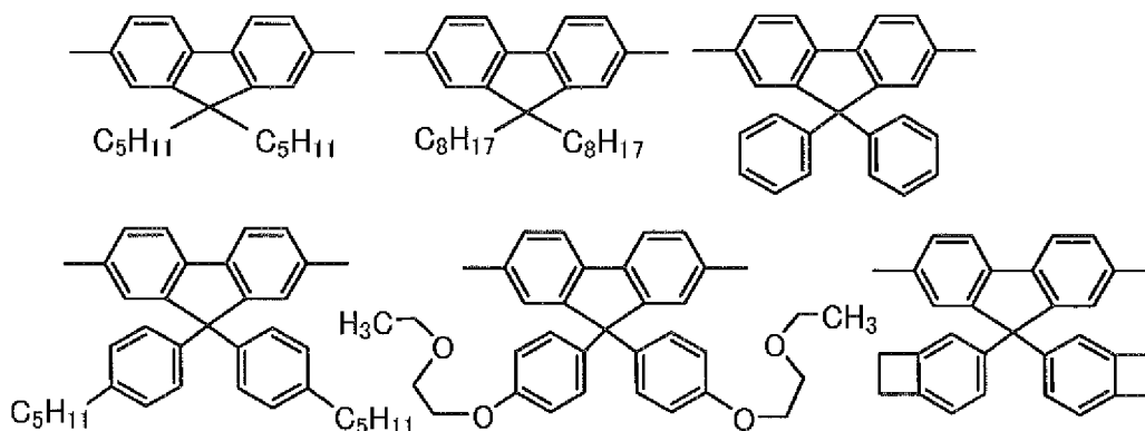
[Chemical Formula 2]
