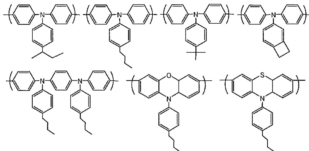
[Chemical Formula 4]
