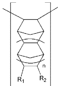
[Chemical Formula 2]
