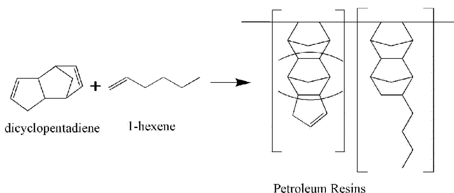
[Reaction Formula 1]
