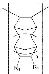
[Chemical Formula 2]
