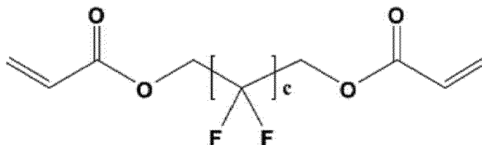
[Chemical Formula 12]
