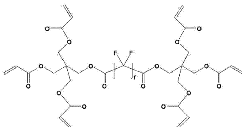
[Chemical Formula 15]
