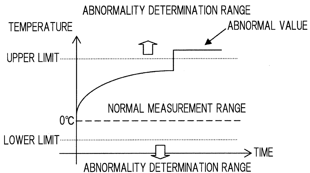
SENSOR ABNORMALITY DETERMINATION EXAMPLE
