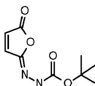
Imine by-product
