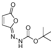
Imine by-product
