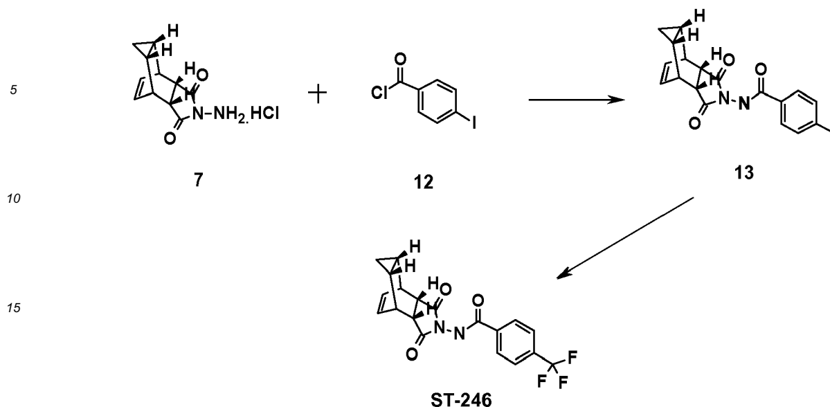
Scheme 5
