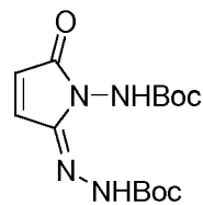
Disubstituted by-product
