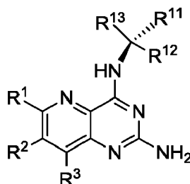
Formula (IVb).
