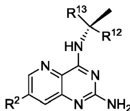
Formula (IVc)
