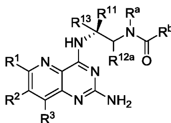
Formula (IVd)
