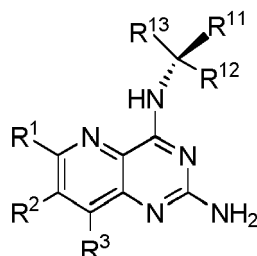
Formula (IVa)
