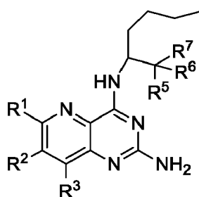
Formula (III)
