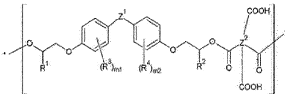
Chemical Formula C
