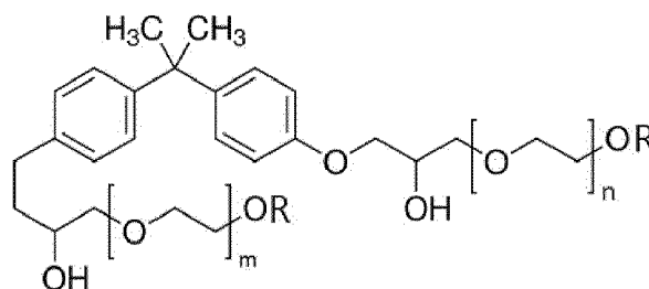
Chemical Formula E-2
