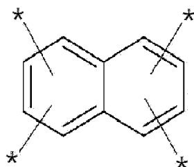
Chemical Formula B-2
