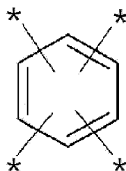
Chemical Formula B-1
