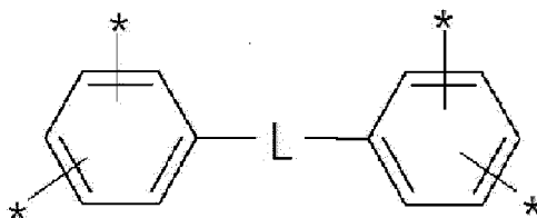
Chemical Formula B-3
