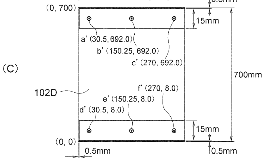
LEFT SIDE PANEL FACE 102D
