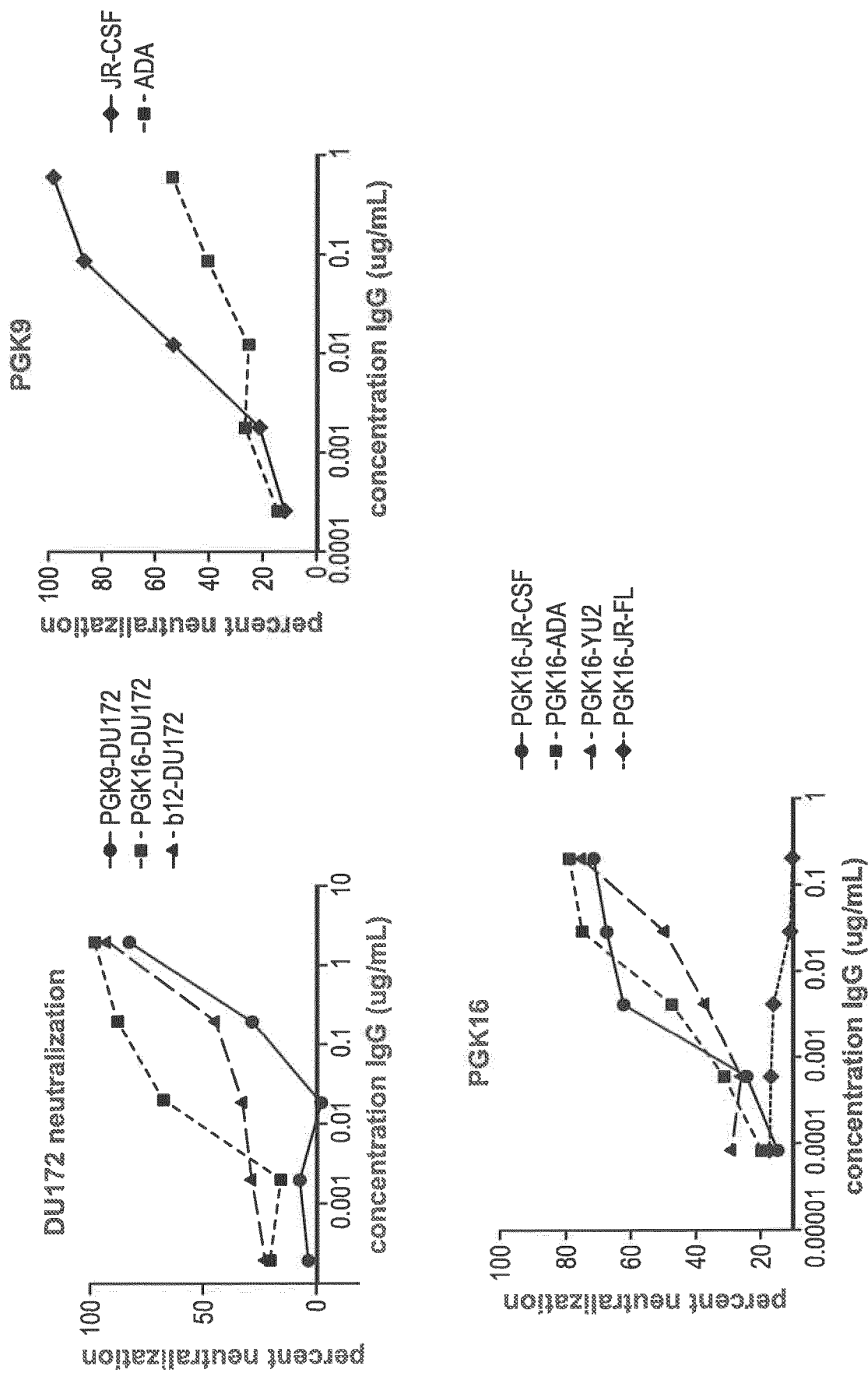
FIG. 4 PG9 and PG16 Neutralization Assays
