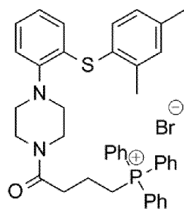
(phosphonium-vortioxetine);
