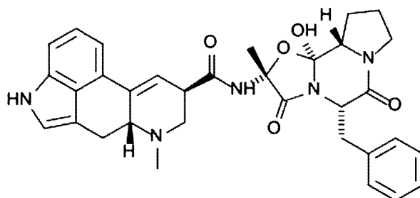
Ergotamine:
