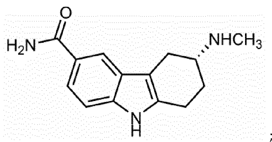
Frovatriptan:
