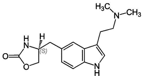
Zolmitriptan:
