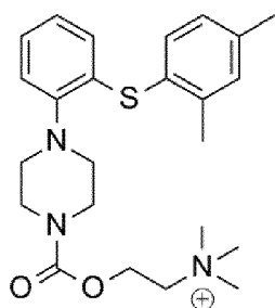
(choline-vortioxetine); Z^-
