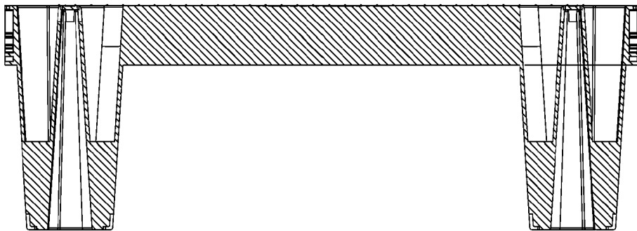
Fig. 82 Section C-C
