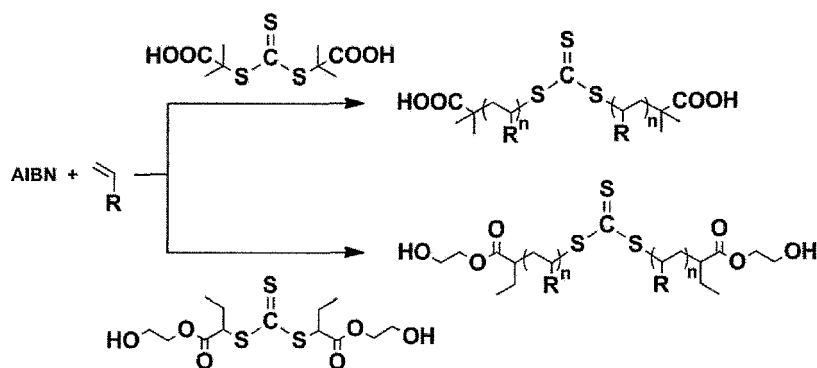
Scheme 1. Schematic showing of the basic mechanism of RAFT polymerization using a telechelic chain transfer agent. AIBN is an exemplary chain initiator, azobisisobutyronitrile; and
