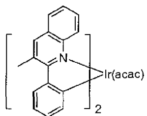
Comp. Ex. 1 \text{Ir}(\text{3-Mepq})_2(\text{acac})
