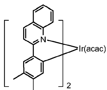
Compound 13
