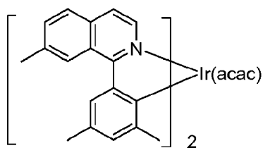
Compound 24
