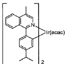
Compound 12
