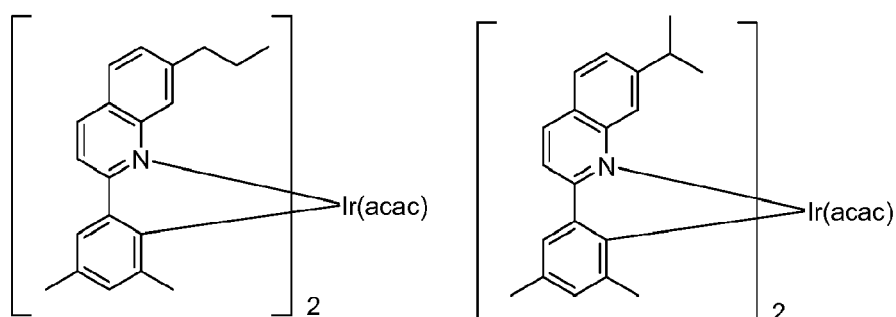
Compound 16
