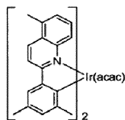
Compound 15
