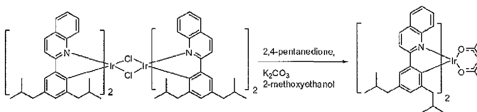
Compound 23
