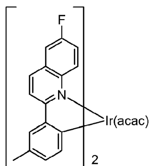
Compound 5
