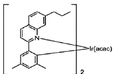
Compound 16
