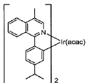
Compound 12
