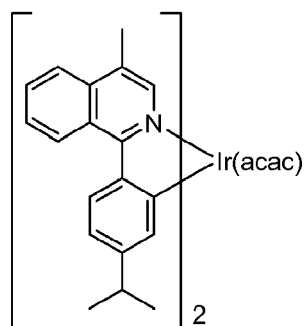
Compound 12
