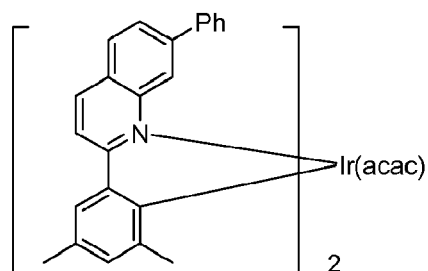
Compound 18 ,
