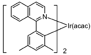
Compound 22 ,
