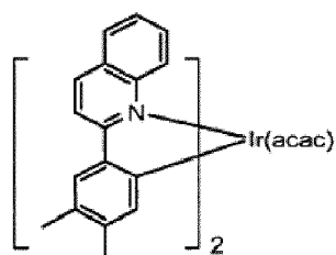
Compound 13
