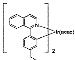
Compound 10
