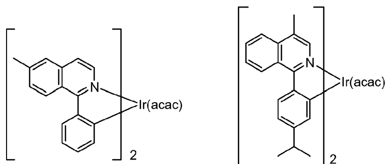
Compound 11
