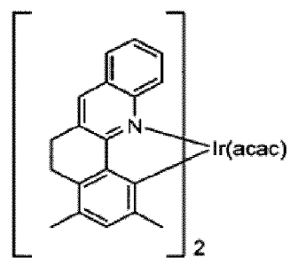
Compound 19
