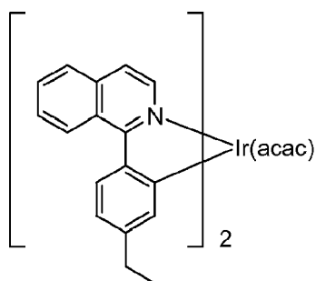
Compound 10
