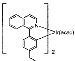
Compound 10
