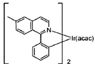
Compound 11
