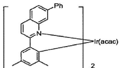
Compound 18
