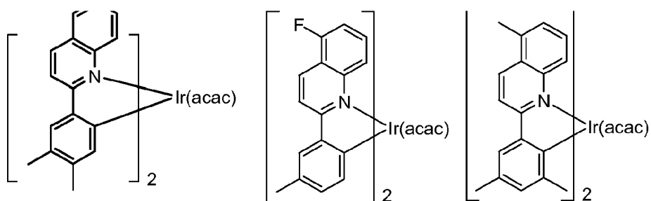
Compound 13
