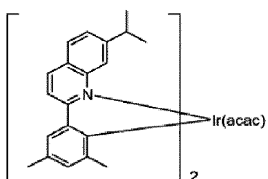
Compound 17
