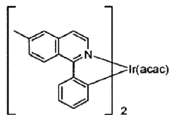
Compound 11
