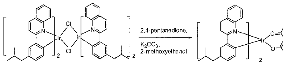
Compound 20
