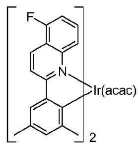
Compound 8
