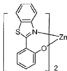
Compound C
