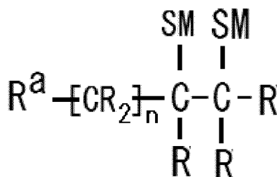
Chemical Formula 2-2
