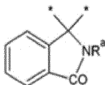
Chemical Formula A-5
