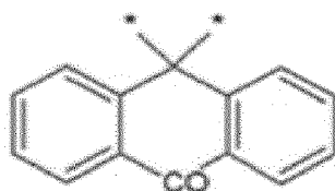
Chemical Formula A-6
