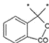
Chemical Formula A-3
