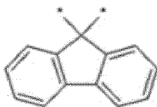
Chemical Formula A-2
