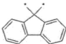
Chemical Formula A-2
