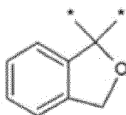
Chemical Formula A-5
