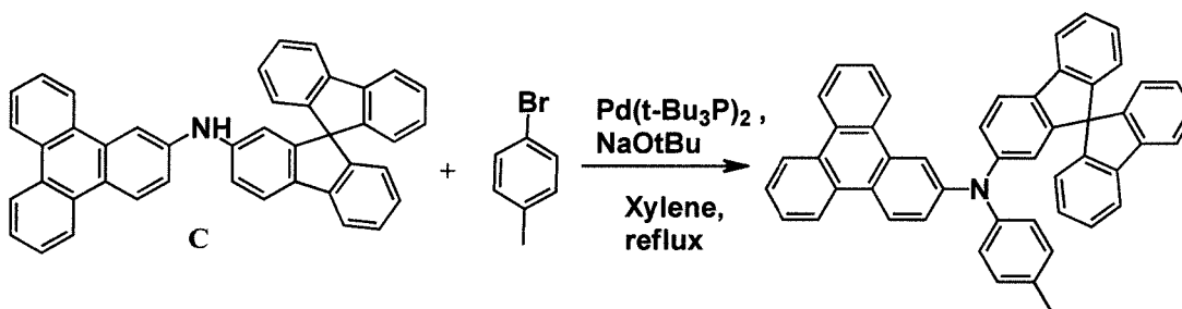
[Compound 1-2]
