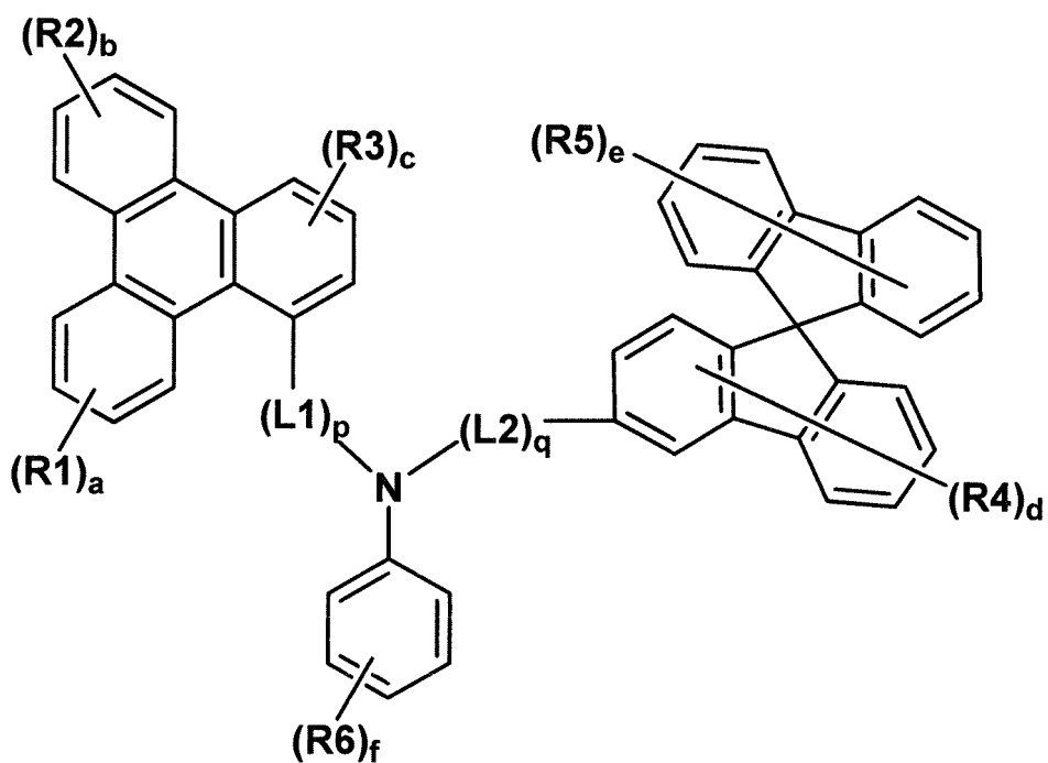
[Chemical Formula 12]
