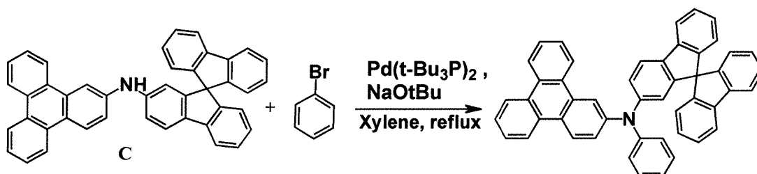
[Compound A]
