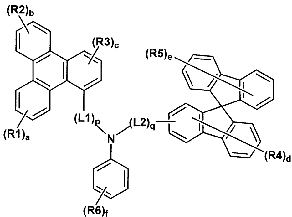
[Chemical Formula 3]
