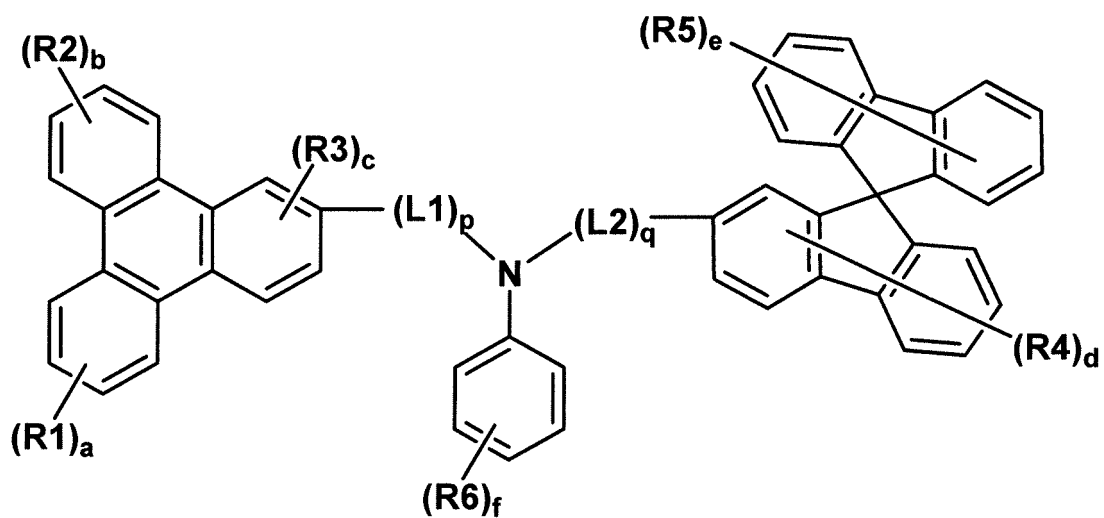
[Chemical Formula 8]
