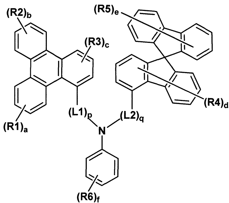
[Chemical Formula 12]
