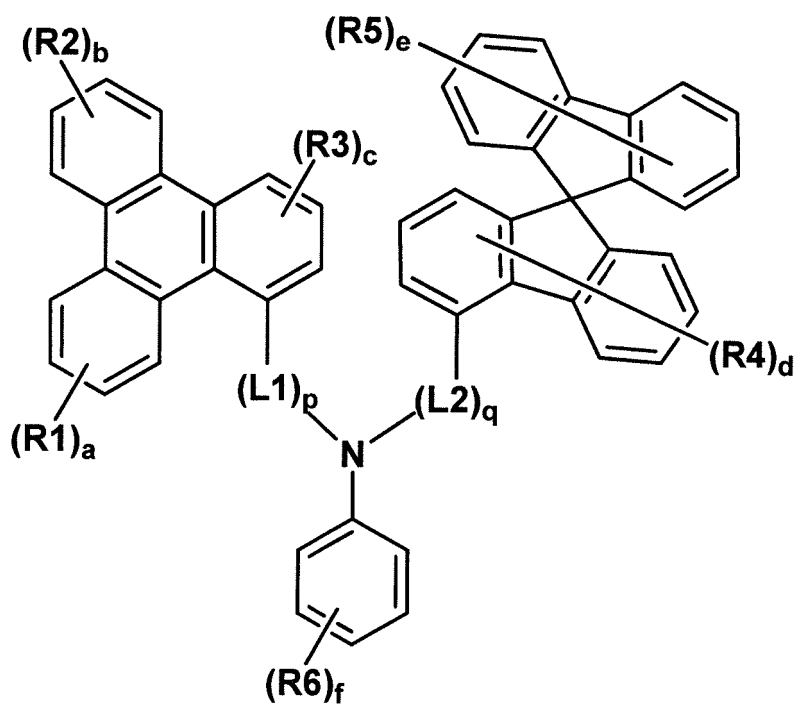
[Chemical Formula 12]
