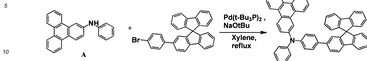
[Compound 1-37]
