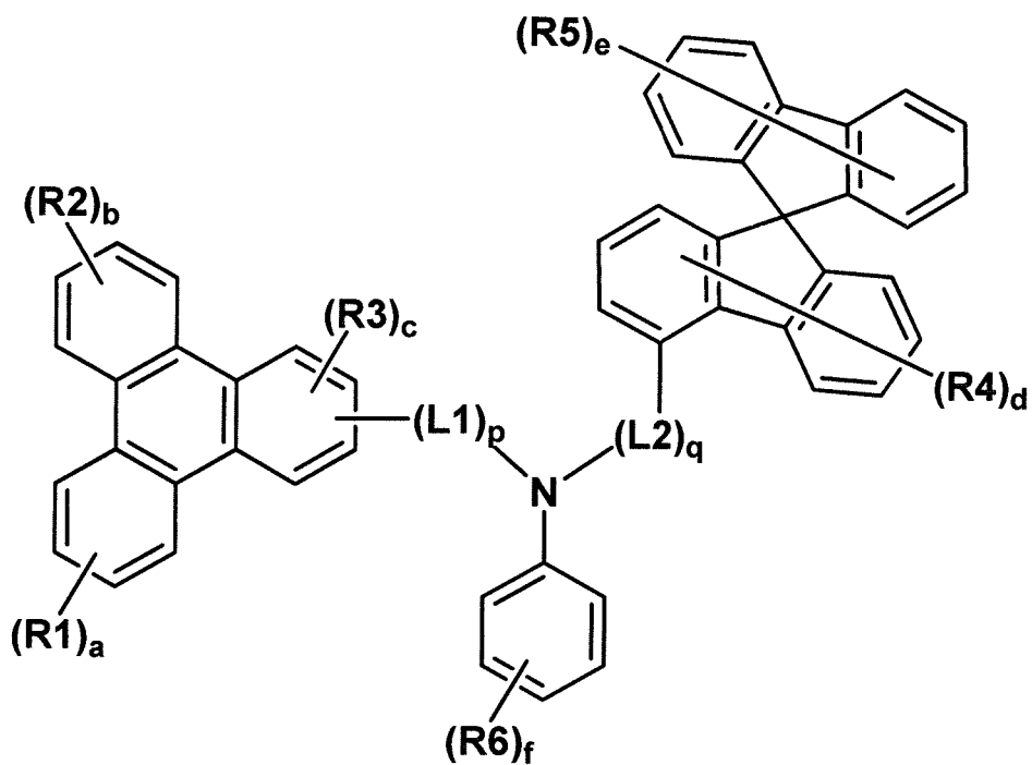
[Chemical Formula 6]
