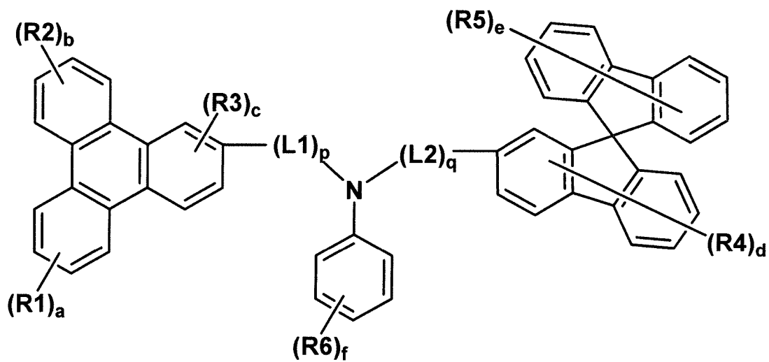
[Chemical Formula 8]
