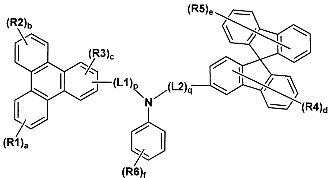
[Chemical Formula 6]
