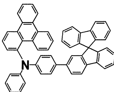
[Compound 1-38]
