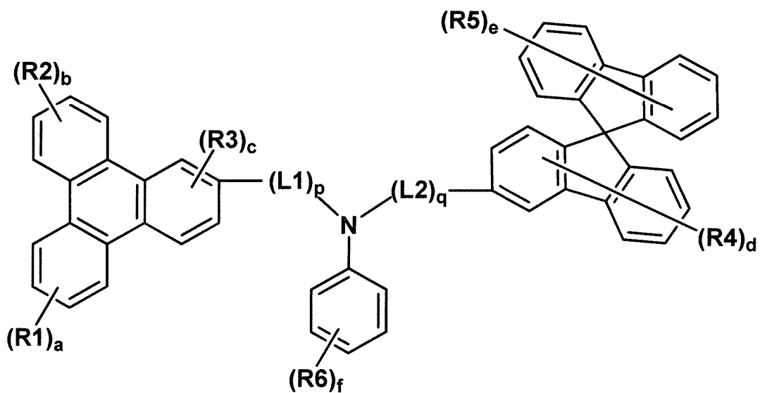
[Chemical Formula 8]
