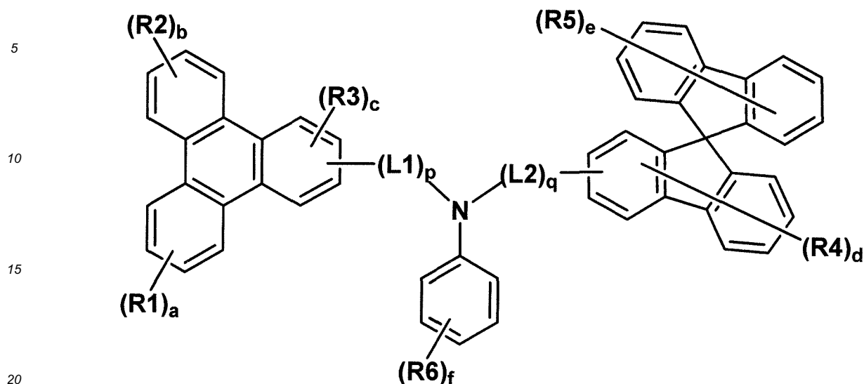
[Chemical Formula 1]
