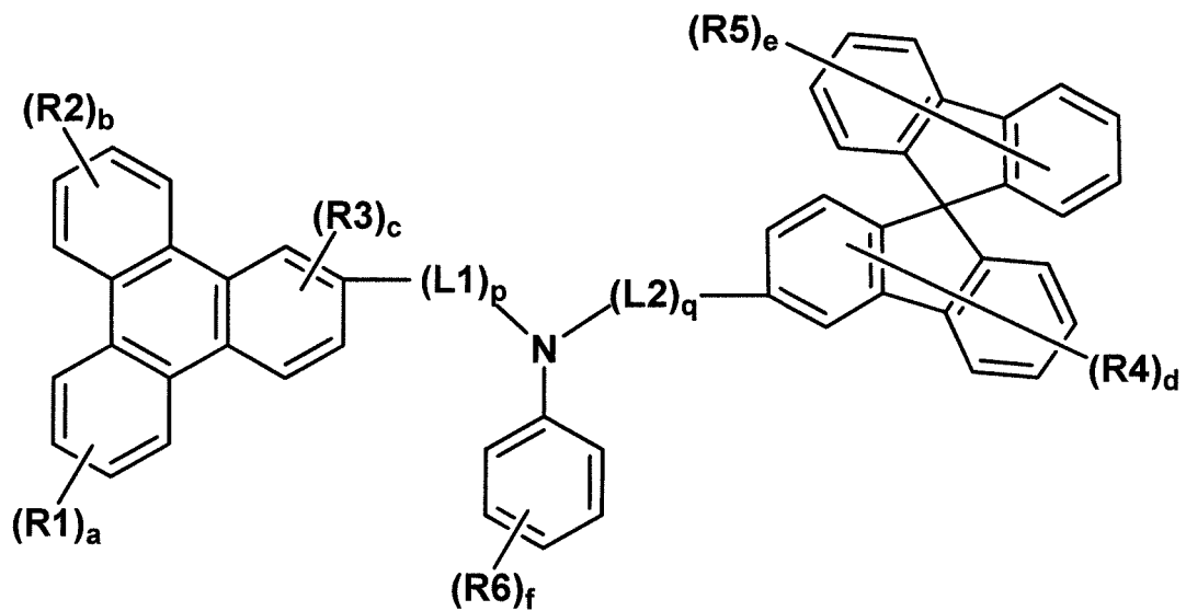
[Chemical Formula 8]
