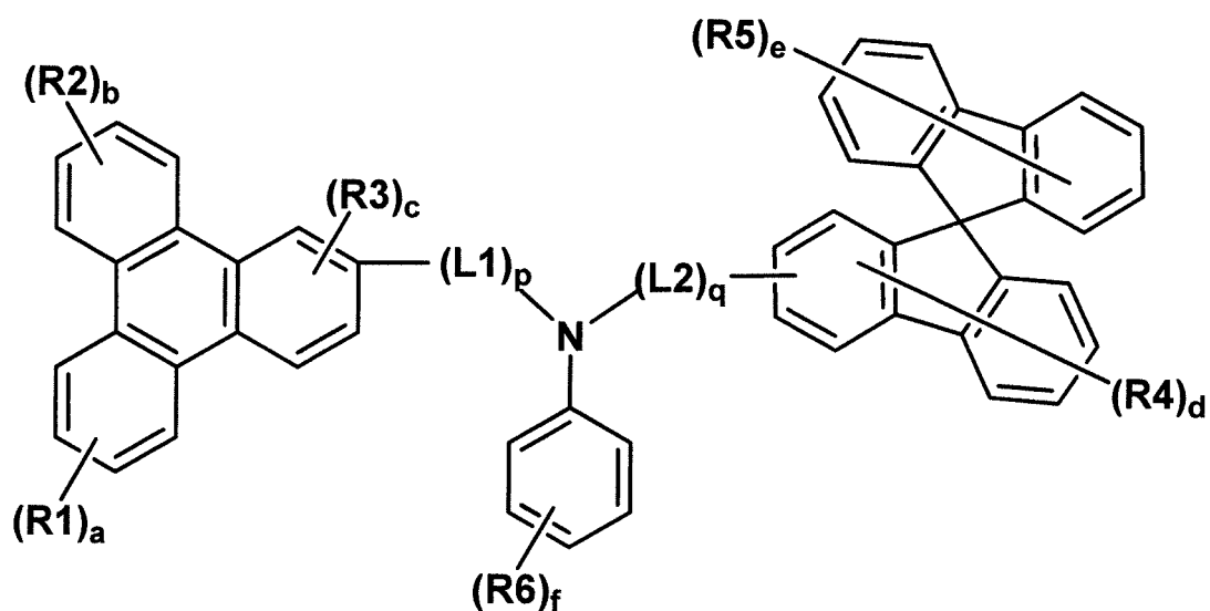
[Chemical Formula 2]
