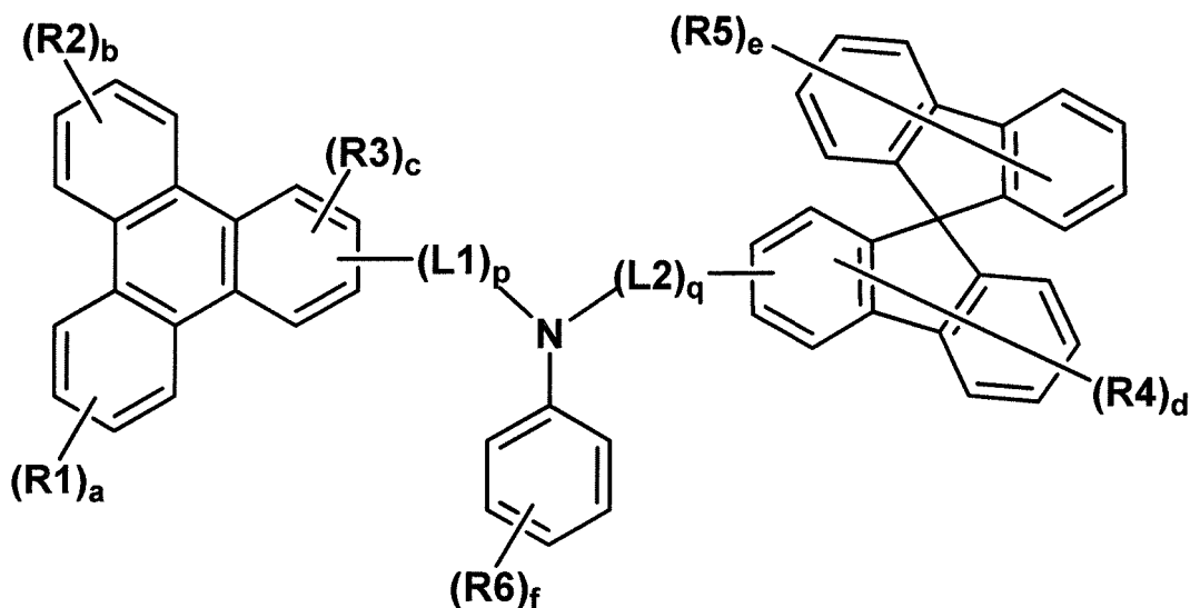
[Chemical Formula 1]
