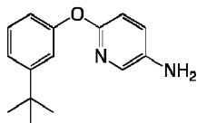
6-(3-(tert-butyl)phenoxy)pyridin-3-amine,
