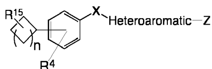
Formula IX
