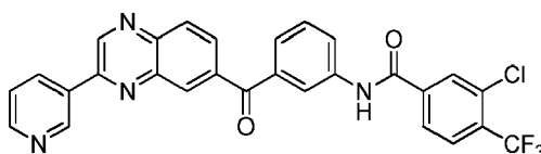
3-chloro-N-(3-(3-(pyridin-3-yl)quinoxaline-6-carbonyl)phenyl)-4-(trifluoromethyl)benzamide
