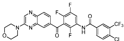
4-chloro-N-(2,4,5-trifluoro-3-(3-morpholinoquinoxaline-6-carbonyl)phenyl)-3-(trifluoromethyl)benzamide
