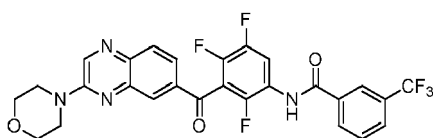
N-(2,4,5-trifluoro-3-(3-morpholinoquinoxaline-6-carbonyl)phenyl)-3-(trifluoromethyl)benzamide
