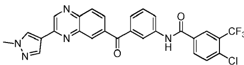
4-chloro-N-(3-(3-(1-methyl-1H-pyrazol-4-yl)quinoxaline-6-carbonyl)phenyl)-3-(trifluoromethyl)benzamide
