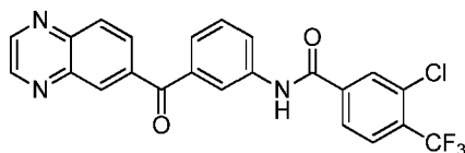
3-chloro- N -(3-(quinoxaline-6-carbonyl)phenyl)-4-(trifluoromethyl)benzamide
