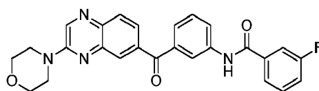
3-fluoro-N-(3-(3-morpholinoquinoxaline-6-carbonyl)phenyl)benzamide
