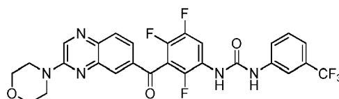
1-(2,4,5-trifluoro-3-(3-morpholinoquinoxaline-6-carbonyl)phenyl)-3-(3-(trifluoromethyl)phenyl)urea
