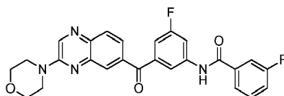
3-fluoro-N-(3-fluoro-5-(3-morpholinoquinoxaline-6-carbonyl)phenyl)benzamide
