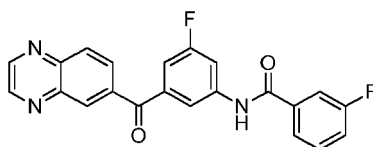
3-fluoro-N-(3-fluoro-5-(quinoxaline-6-carbonyl)phenyl)benzamide
