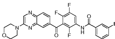
3-fluoro-N-(2,4,5-trifluoro-3-(3-morpholinoquinoxaline-6-carbonyl)phenyl)benzamide
