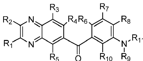
Formula I
