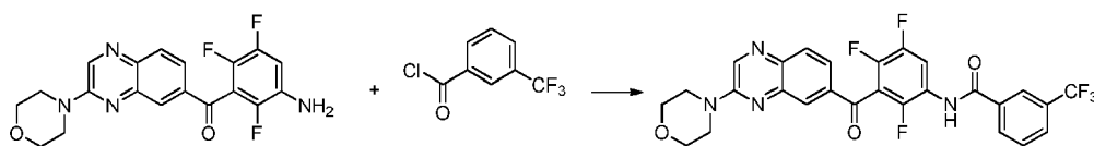
N-(2,4,5-trifluoro-3-(3-morpholinoquinoxaline-6-carbonyl)phenyl)-3-(trifluoromethyl)benzamide
