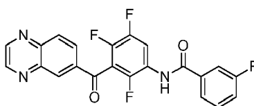
3-fluoro-N-(2,4,5-trifluoro-3-(quinoxaline-6-carbonyl)phenyl)benzamide
