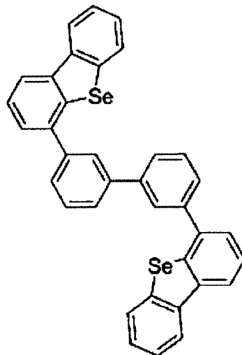
Comparative compound 4
