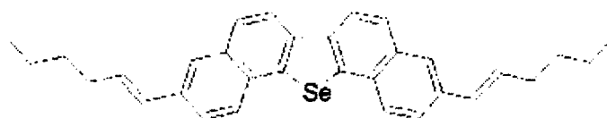
Compound 8
