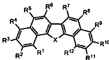
General Formula (1)
