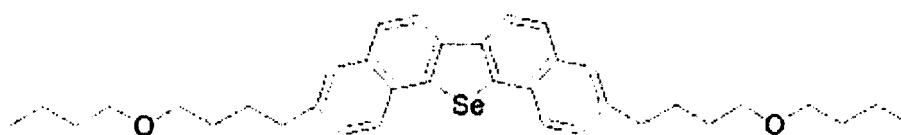
Compound 6
