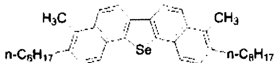
Compound 5
