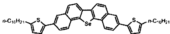
Compound 4
