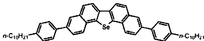
Compound 3
