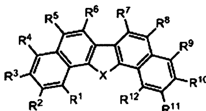
General Formula (1)
