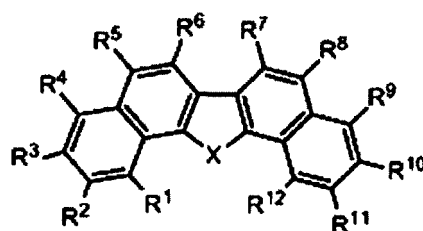
General Formula (1)
