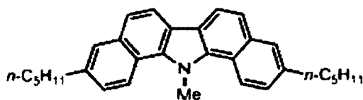
Comparative compound 3
