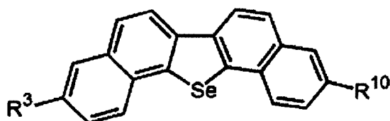
General Formula (2)
