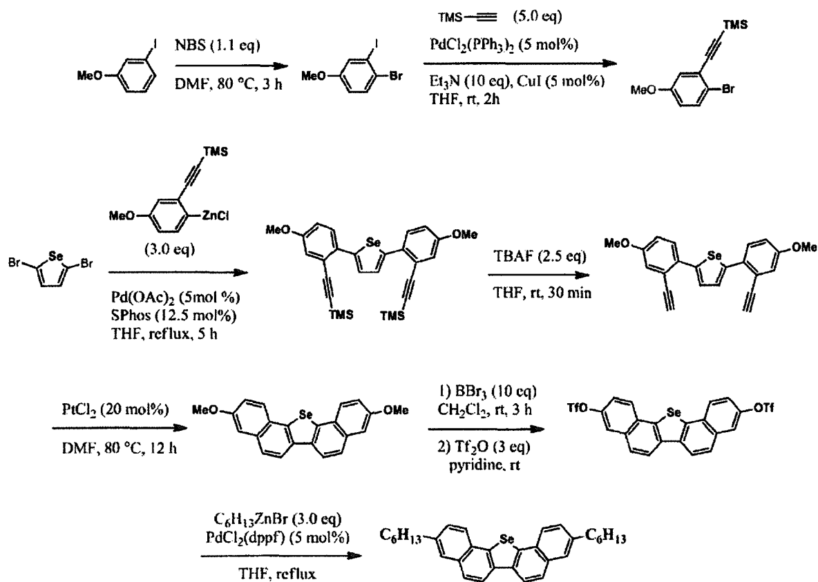
Compound 1
