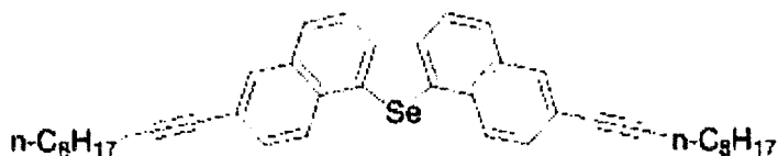
Compound 7
