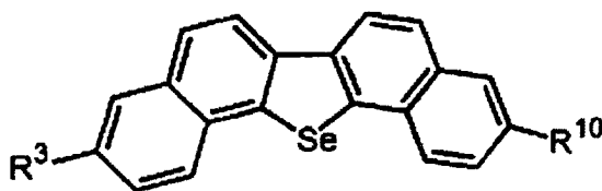
General Formula (2)
