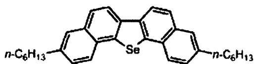
Compound 1
