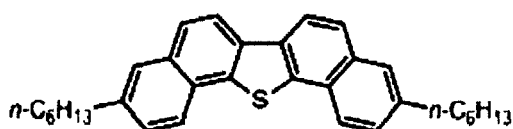
Comparative compound 2
