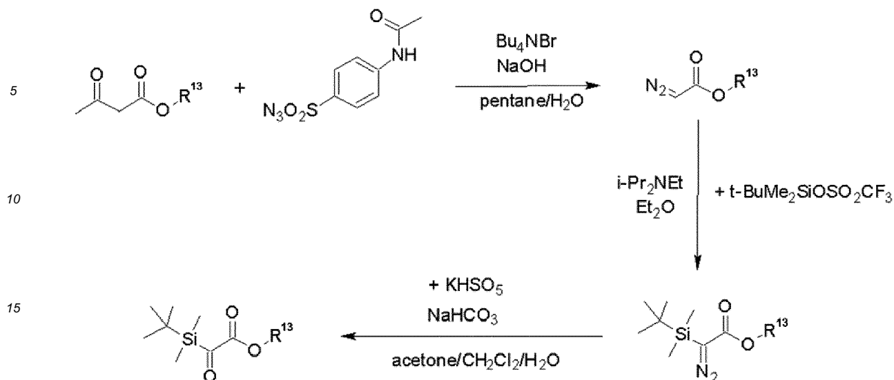
Scheme 4: Preparation of silylglyoxylates
