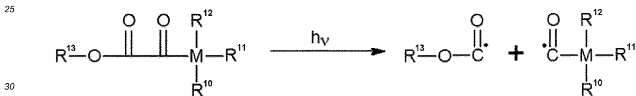
Scheme 6: Cleavage of -O-C(=O)-C(=O)- moiety of a glyoxylate
