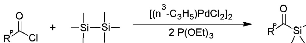
Scheme 3: Preparation of acylsilanes
