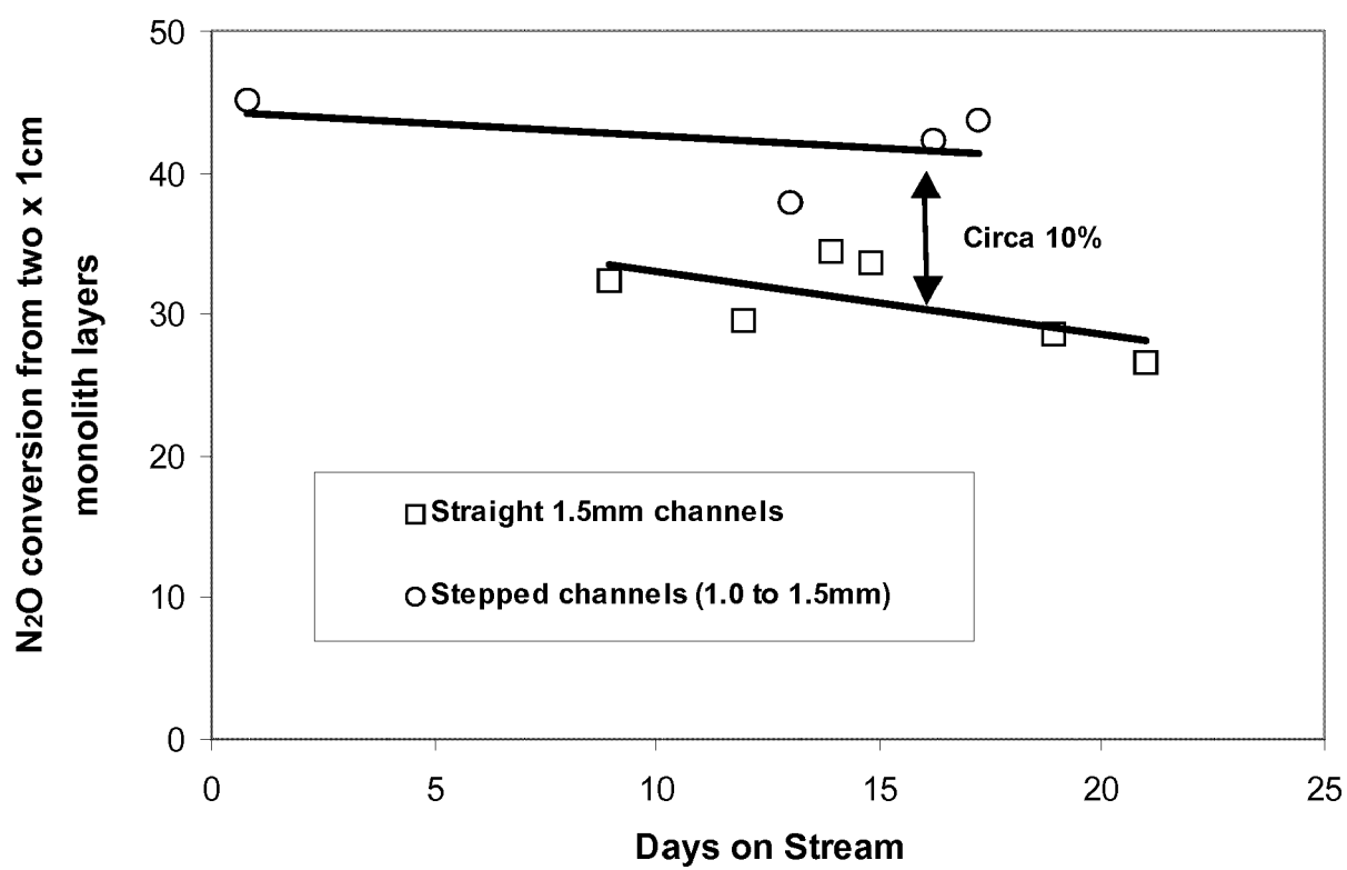
Fig. 14. N 2 O conversion over straight and stepped-channel monoliths
