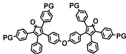
(1d) PG = CO 2 H; (1e) PG = OH
