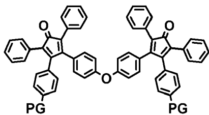
(1b) PG = CO 2 H; (1c) PG = OH
