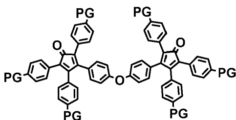
(1f) PG = CO 2 H; (1g) PG = OH
