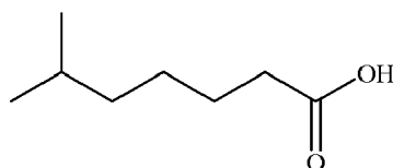
2,2-dimethyloctanoic acid
