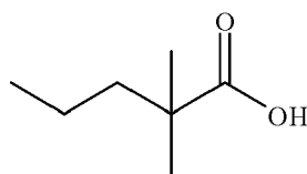
2,2-dimethylpentanoic acid
