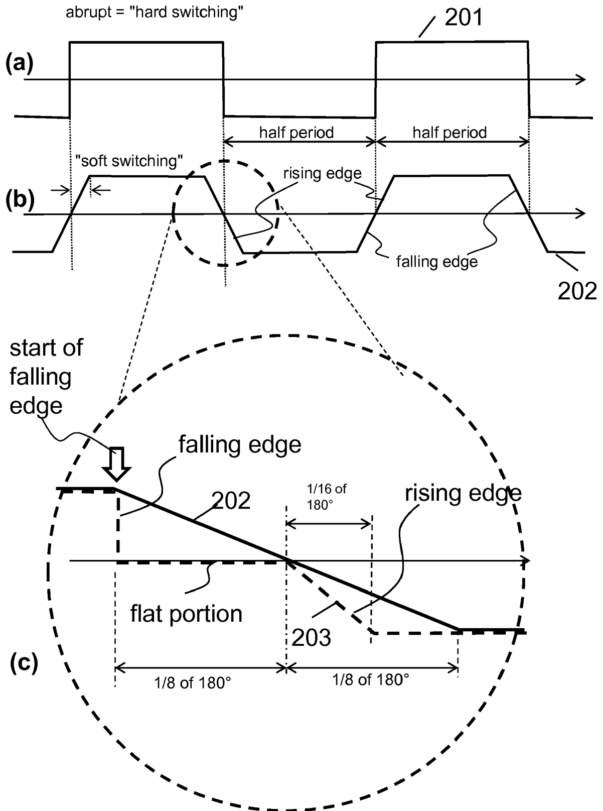
FIG 2 (prior art)
