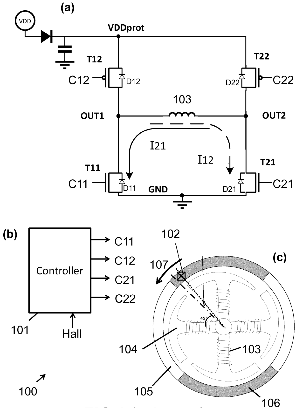
FIG 1 (prior art)
