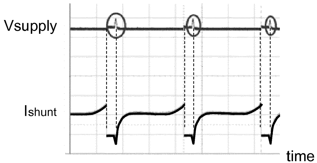
FIG 4 (prior art)
