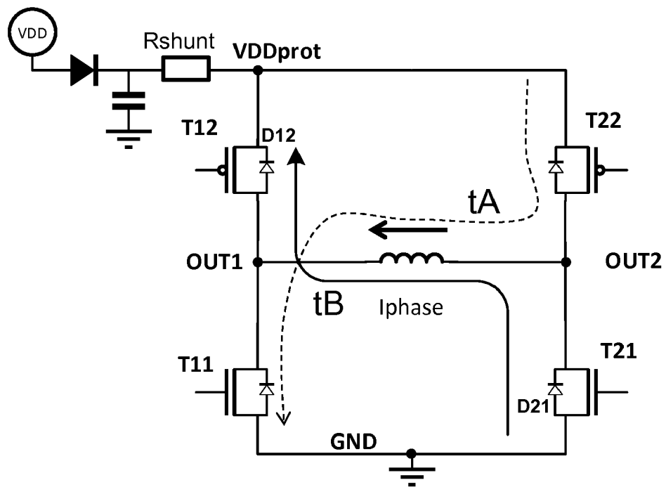
FIG 3 (prior art)
