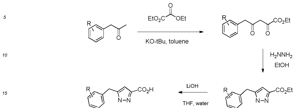
Scheme 7
