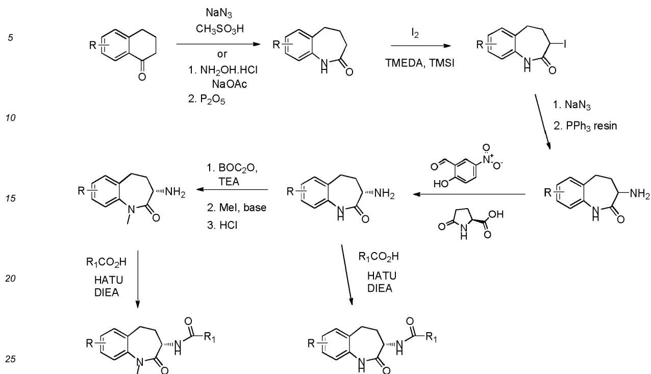
Scheme 5
