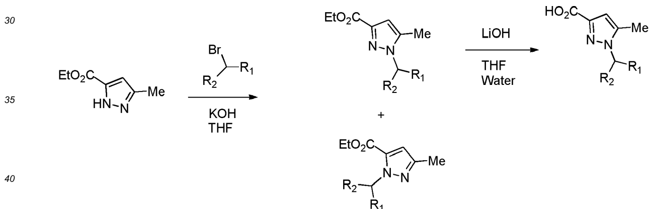
Scheme 8
