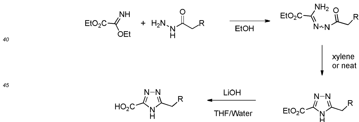
Scheme 6
