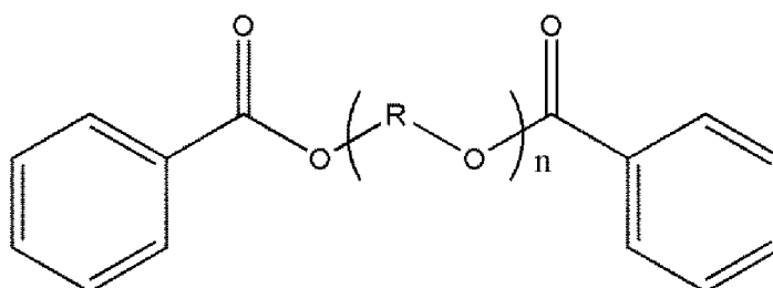
[Chemical Formula 2]
