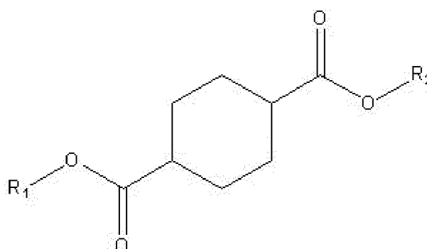
[Chemical Formula 1]
