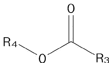
[Chemical Formula 2]
