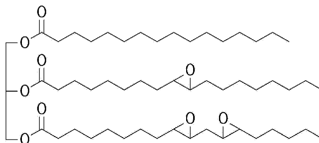
[Chemical Formula 4]
