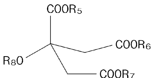
[Chemical Formula 3]
