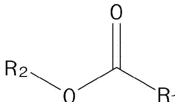
[Chemical Formula 1]
