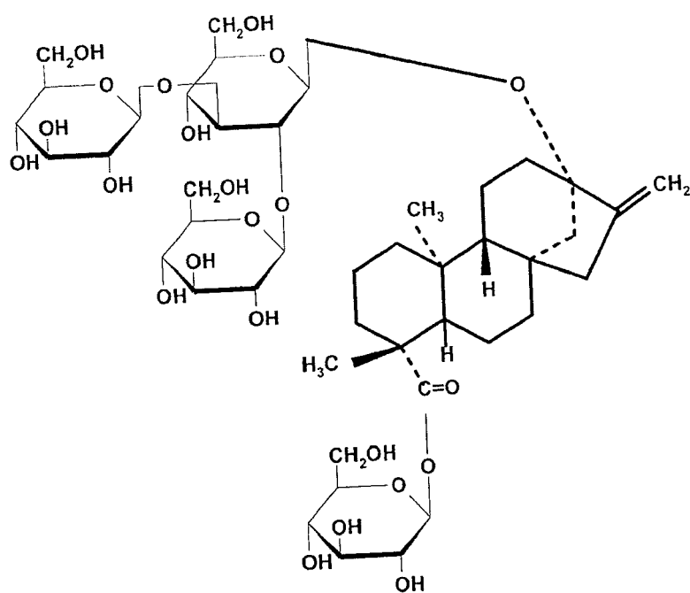
Rebaudioside A
