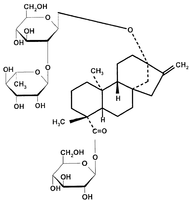
Dulcoside A
