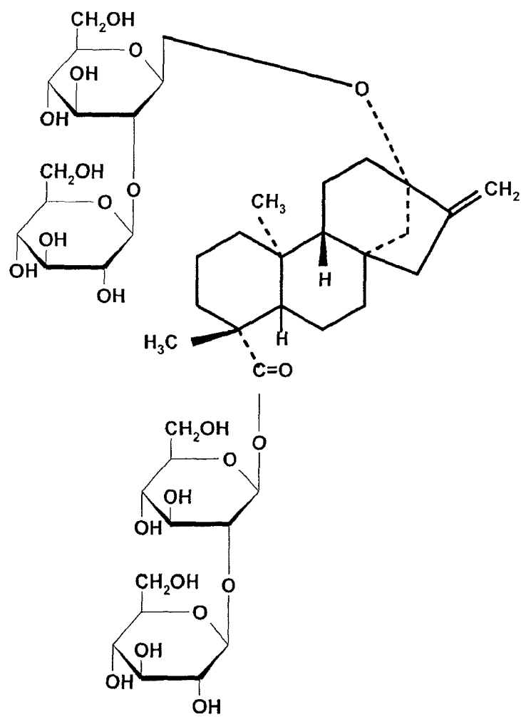
Rebaudioside E
