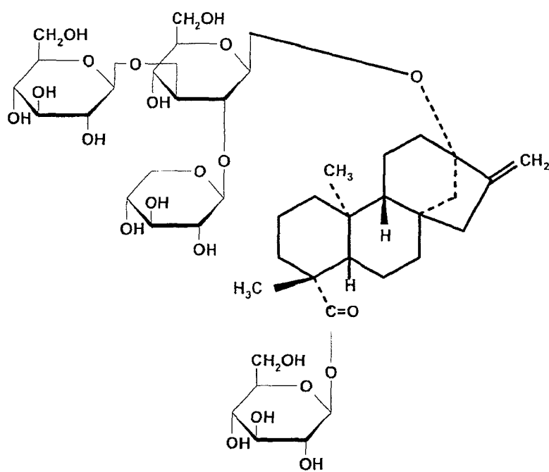
Rebaudioside F
