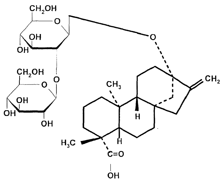
Steviolbioside
