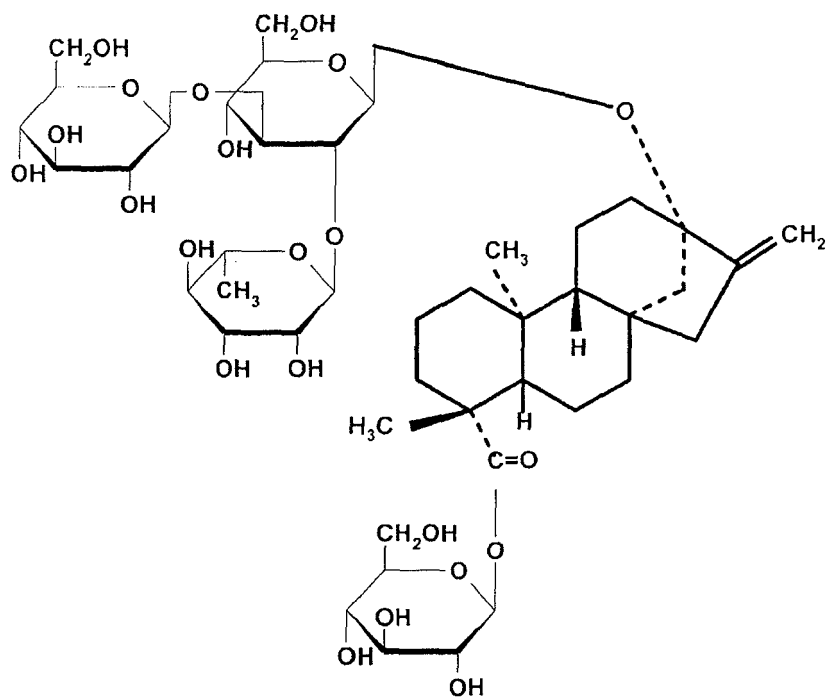
Rebaudioside C
