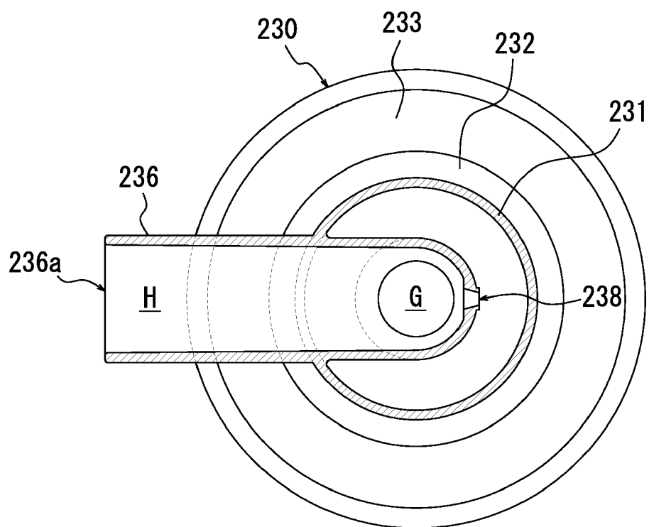
D-D Sectional View
