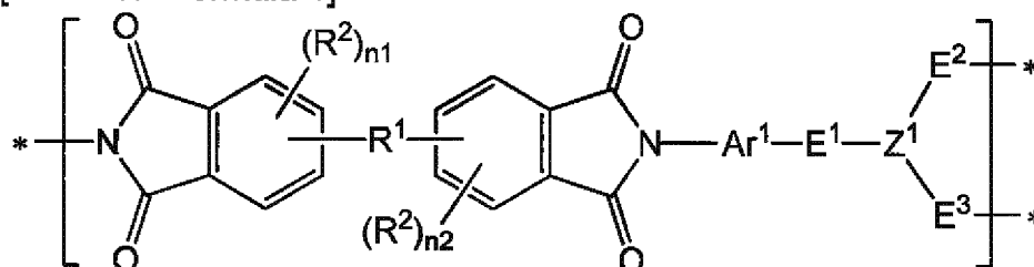
[Chemical Formula 1]
