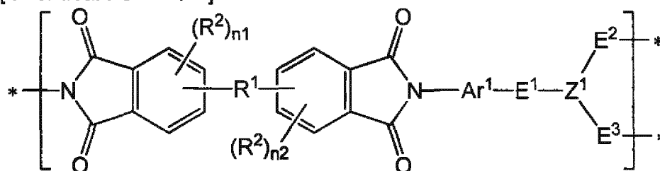
[Chemical Formula 1]
